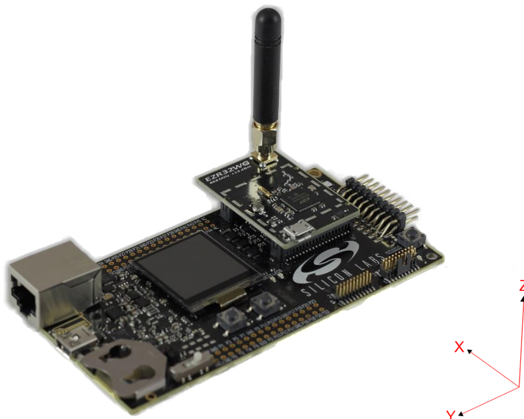
Figure 6.2. DUT: BRD4505B (Rev. A00) Radio Board with Wireless Starter Kit Mainboard
