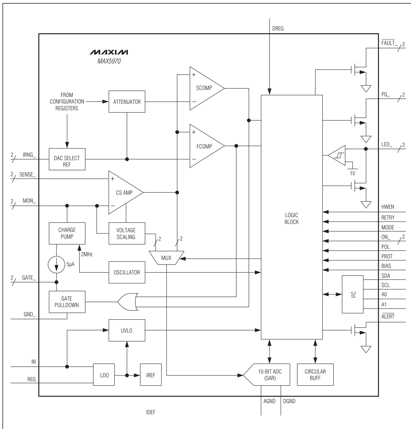
Block Diagram
