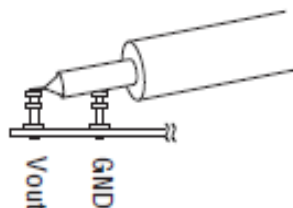
Figure 4. Proper Input/Output Ripple Measurement Technique
