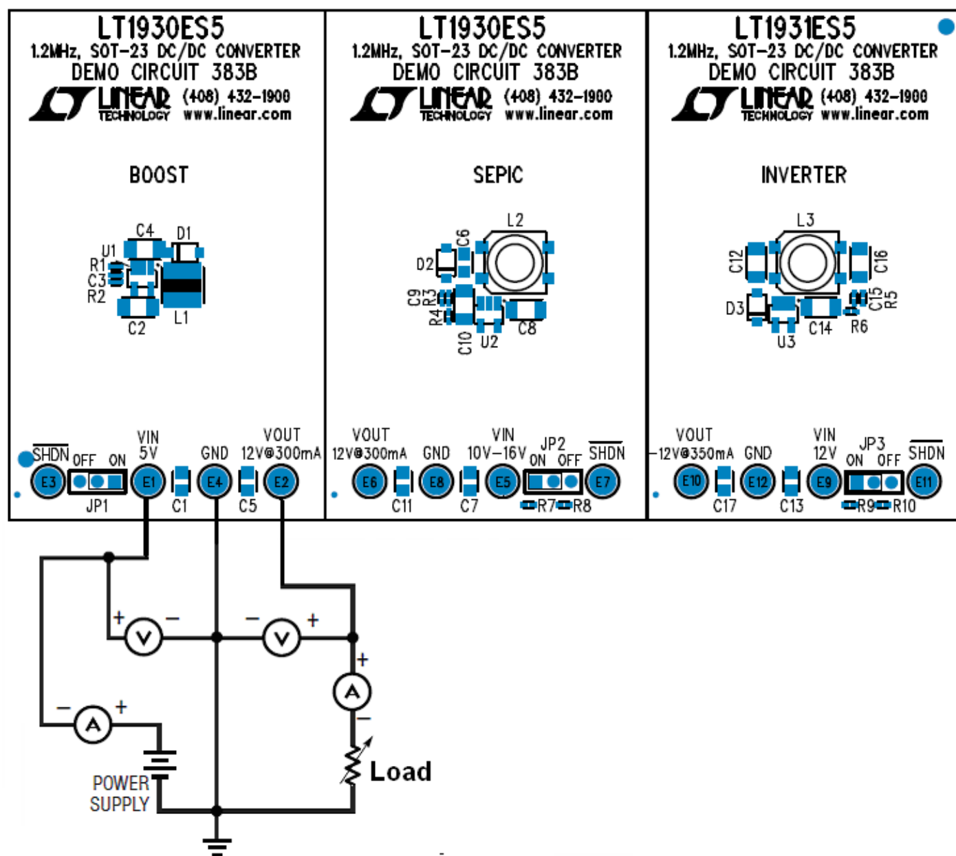
Figure 1. Proper Measurement Equipment Setup for Boost Converter
