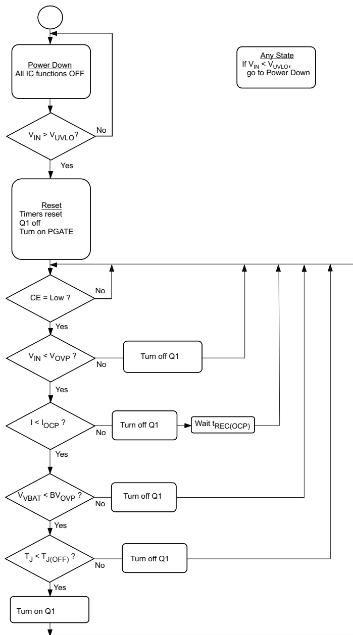
Figure 10. State Diagram
