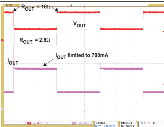
Figure 20. OCP, Showing Current Limiting
