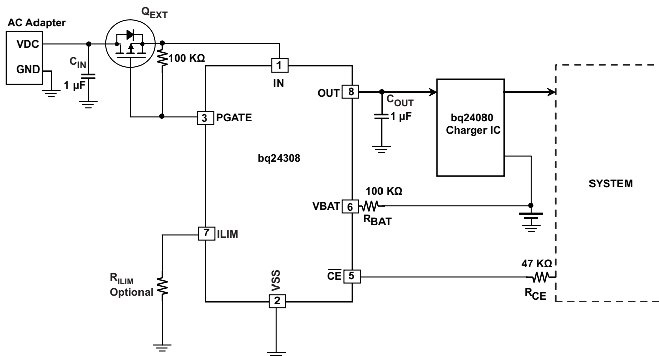
Figure 13. OVP, OCP, BATOVP With Input Reverse-Polarity Protection
