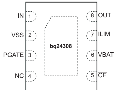
Pin Functions
