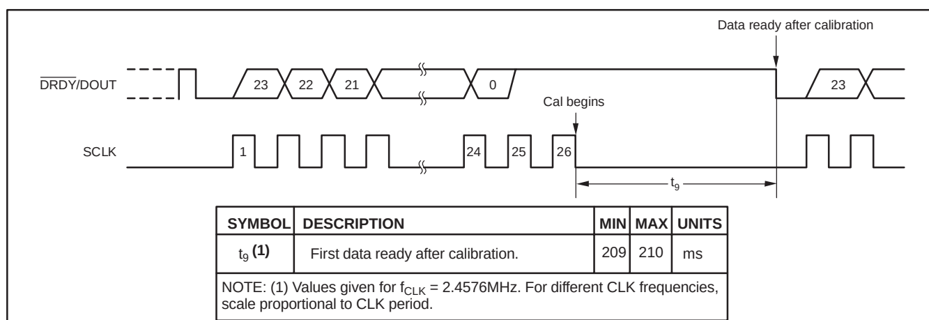
Figure 26. Self-Calibration Timing
