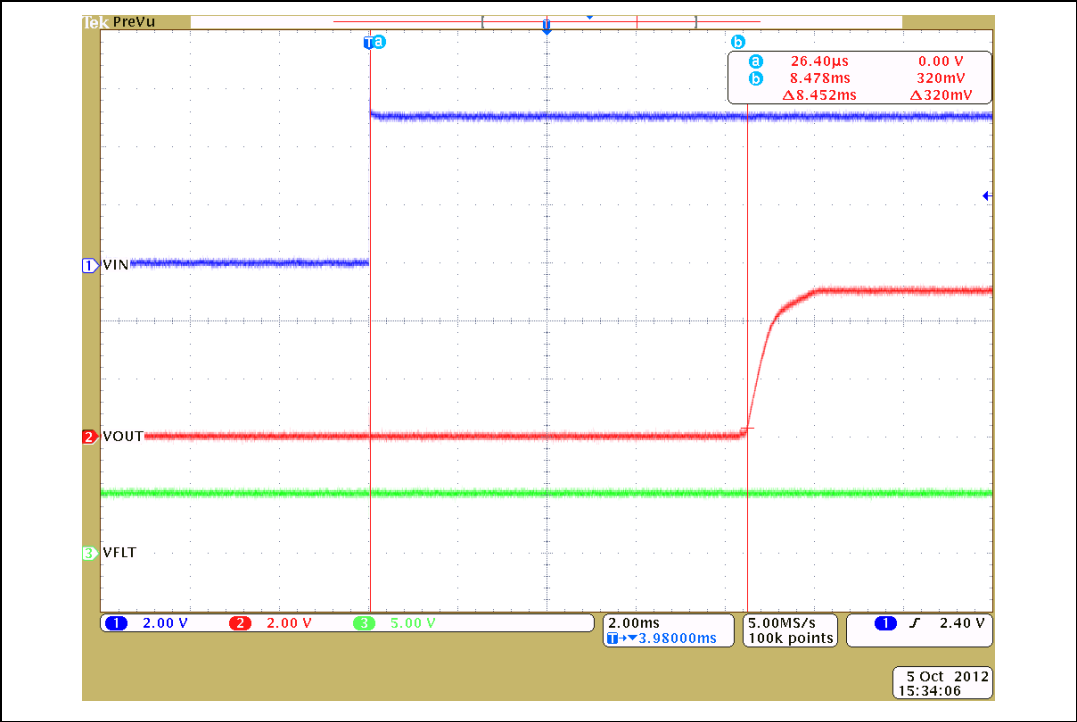
Figure 11. Startup, t_{on}
