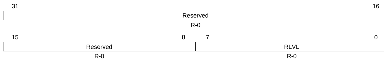
Figure 19-81. Read FIFO Status Register (RFIFOSTS)
