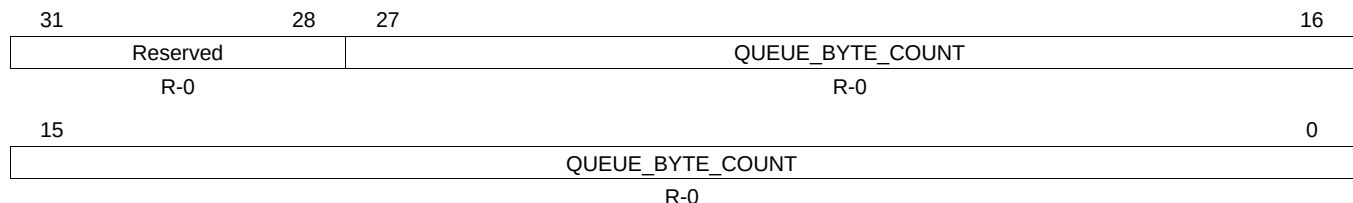
Figure 25-116. Queue Manager Queue N Status Register B (QSTATB[N])
