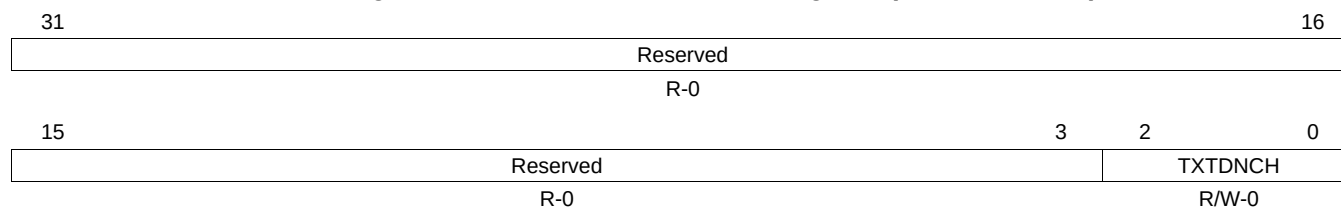
Figure 15-41. Transmit Teardown Register (TXTEARDOWN)
