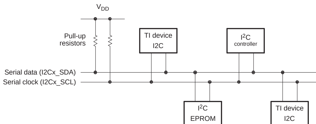
Figure 18-2. Multiple I2C Modules Connected
