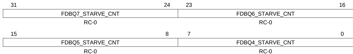
Figure 25-104. Queue Manager Free Descriptor/Buffer Starvation Count Register 1 (FDBSC1)
