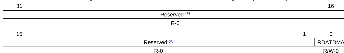
Figure 19-57. Receiver DMA Event Control Register (REVTCTL)
