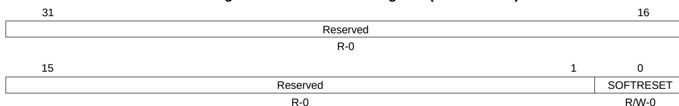
Figure 15-72. Soft Reset Register (SOFTRESET)
