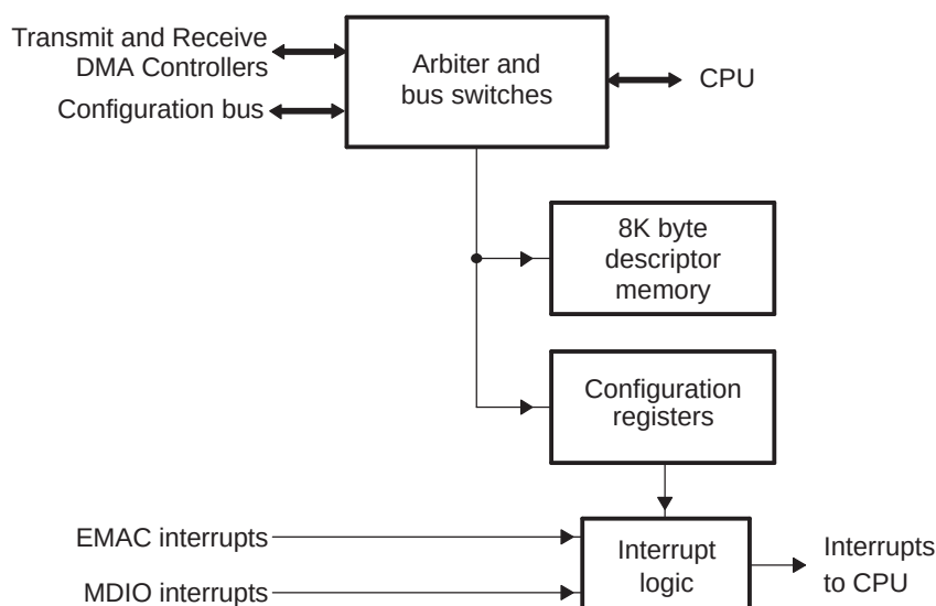
Figure 15-9. EMAC Control Module Block Diagram
