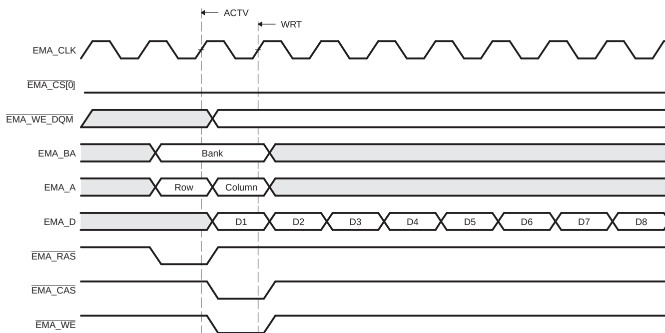
Figure 16-6. Timing Waveform for Basic SDRAM Write Operation
