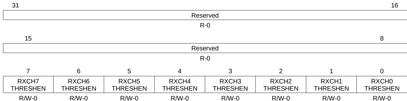
Figure 15-15. EMAC Control Module Interrupt Core 0-2 Receive Threshold Interrupt Enable Register (CnRXTHRESHEN)
