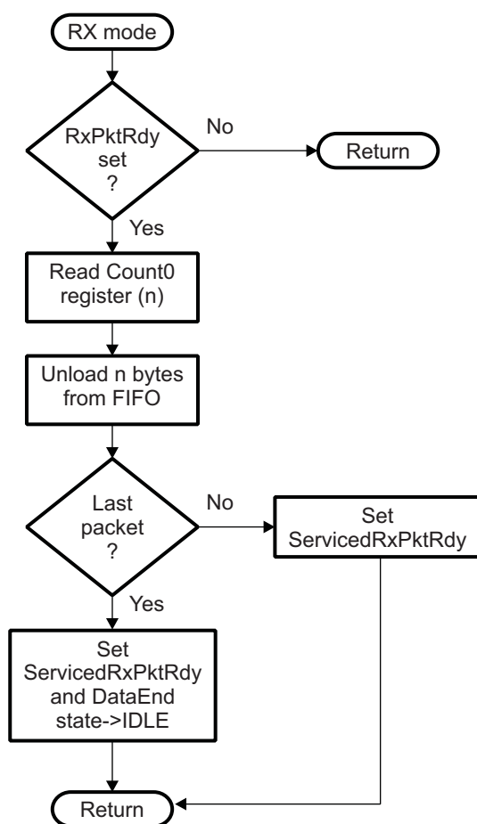
Figure 25-9. RX Mode Flow Chart
