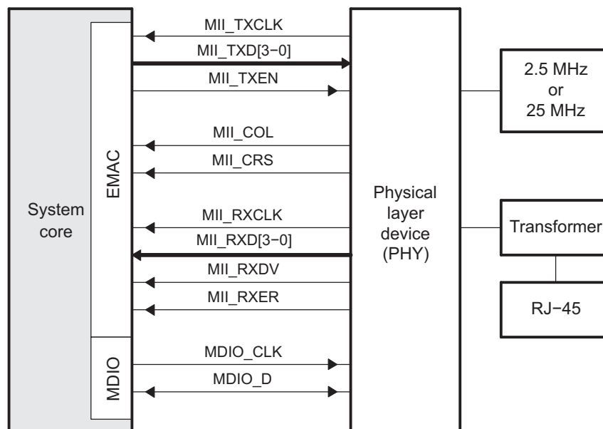
Figure 15-2. Ethernet Configuration—MII Connections
