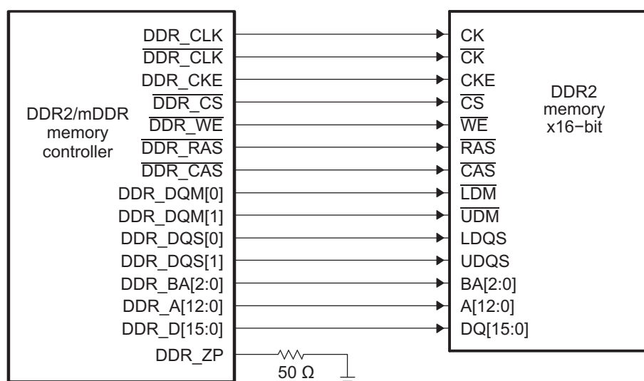
Figure 13-18. Connecting DDR2/mDDR Memory Controller to a 16-Bit DDR2 Memory
