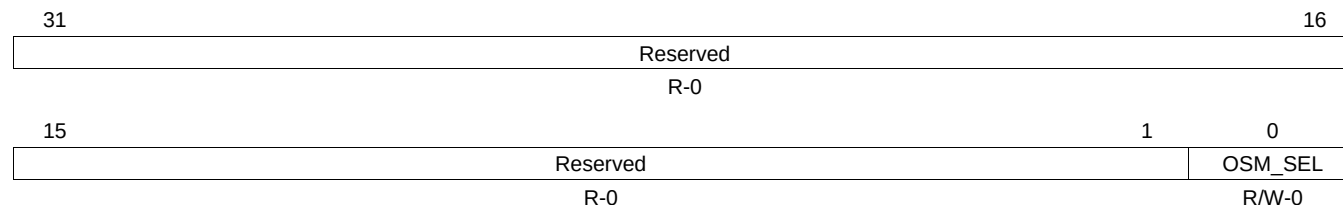
Figure 24-24. Mode Definition Register (MDR)
