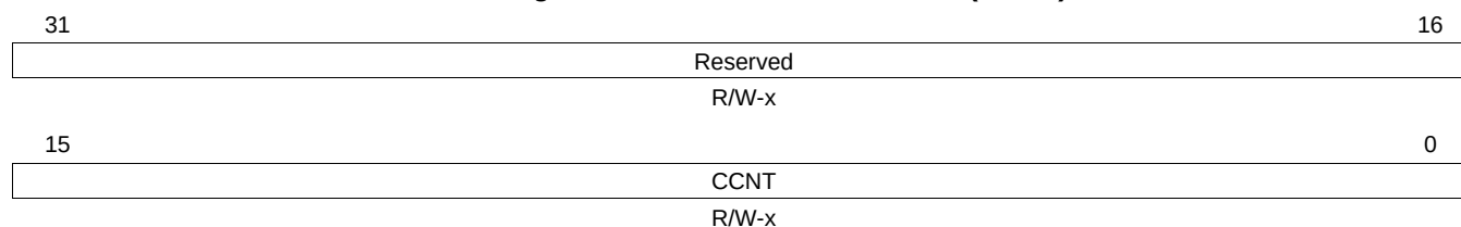
Figure 14-42. C Count Parameter (CCNT)
