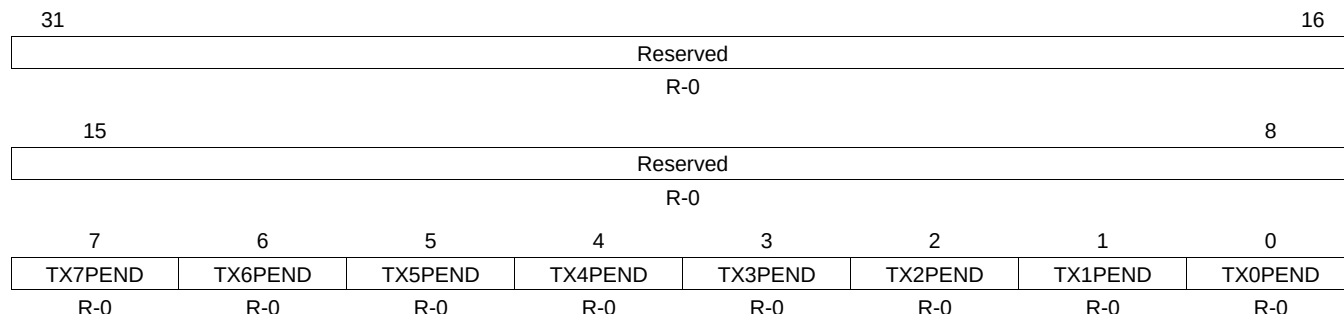
Figure 15-46. Transmit Interrupt Status (Masked) Register (TXINTSTATMASKED)
