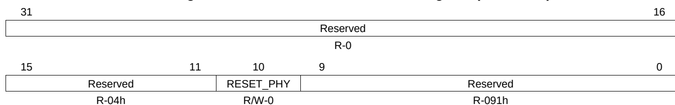
Figure 13-32. DDR PHY Reset Control Register (DRPYRCR)
