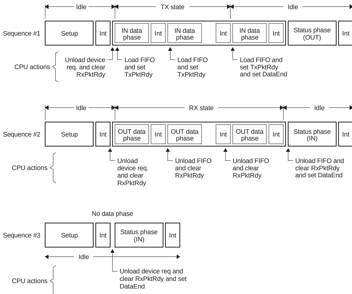
Figure 25-5. Sequence of Transfer
