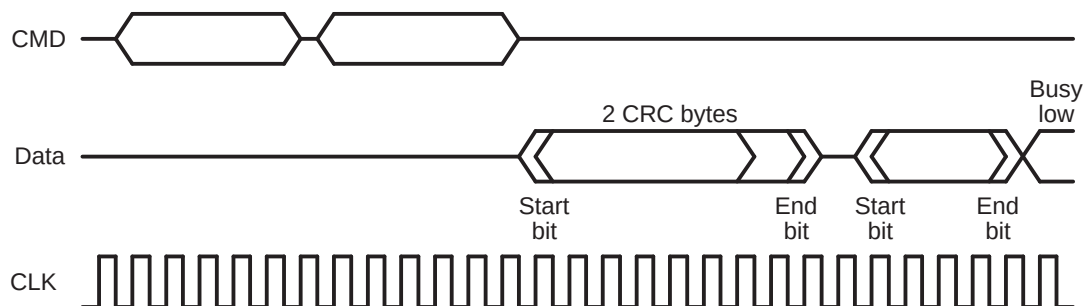
Figure 20-5. MMC/SD Mode Write Sequence Timing Diagram
