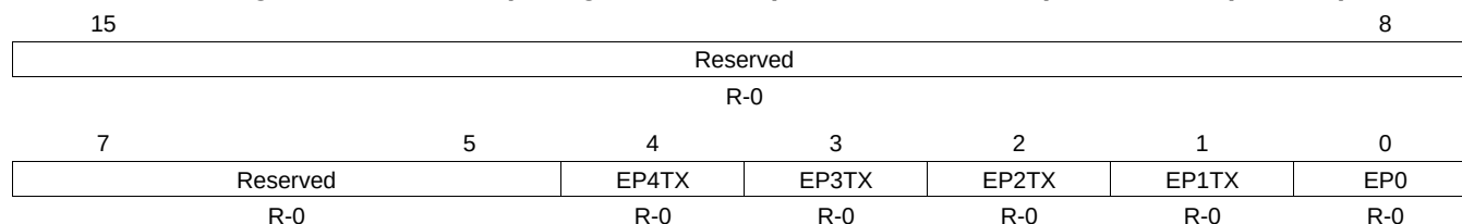
Figure 25-49. Interrupt Register for Endpoint 0 Plus Tx Endpoints 1 to 4 (INTRTX)
