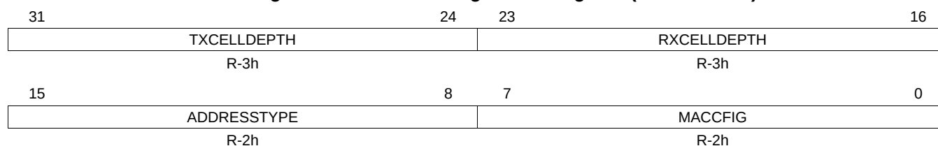
Figure 15-71. MAC Configuration Register (MACCONFIG)
