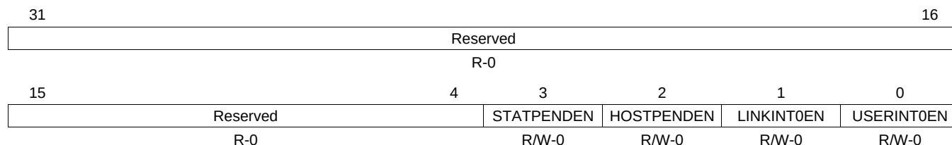
Figure 15-18. EMAC Control Module Interrupt Core 0-2 Miscellaneous Interrupt Enable Register (CnMISCEN)
