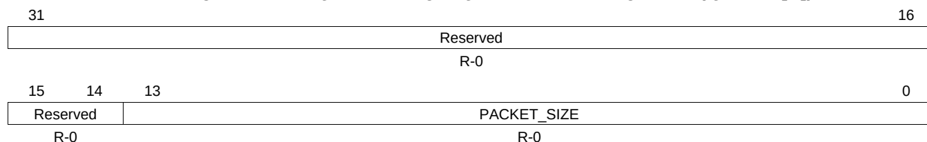
Figure 25-117. Queue Manager Queue N Status Register C (QSTATC[ N ])
