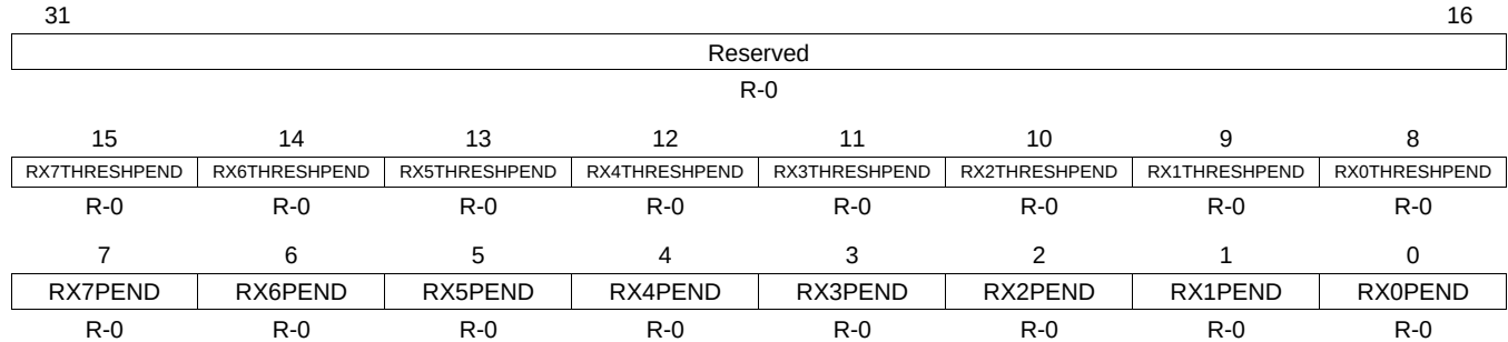
Figure 15-51. Receive Interrupt Status (Unmasked) Register (RXINTSTATRAW)
