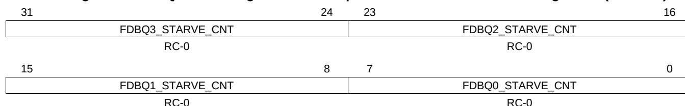
Figure 25-103. Queue Manager Free Descriptor/Buffer Starvation Count Register 0 (FDBSC0)
