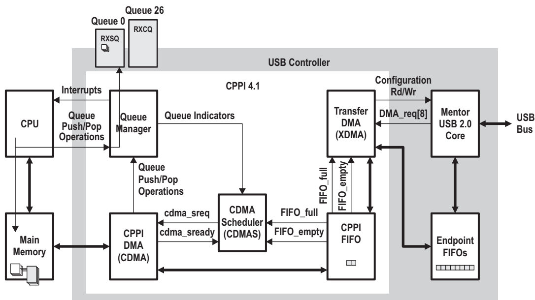
Figure 25-25. Receive USB Data Flow Example (Initialization)
