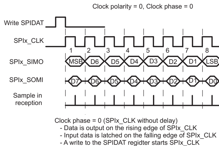
Figure 22-8. Clock Mode with POLARITY = 0 and PHASE = 0
