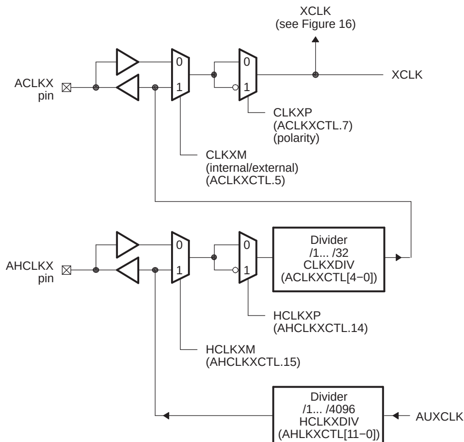
Figure 19-15. Transmit Clock Generator Block Diagram
