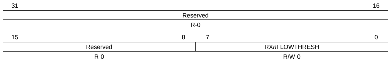
Figure 15-65. Receive Channel n Flow Control Threshold Register (RX n FLOWTHRESH)
