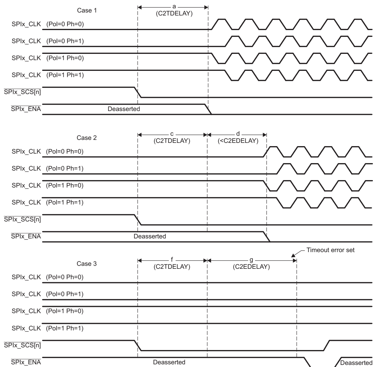
Figure 22-17. SPI 5-Pin Mode Demonstrating C2TDELAY and C2EDELAY
