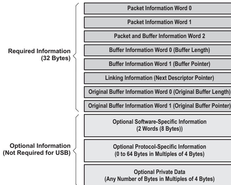
Figure 25-16. Host Packet Descriptor Layout
