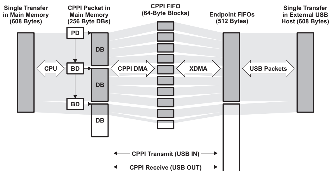
Figure 25-20. High-Level Transmit and Receive Data Transfer Example
