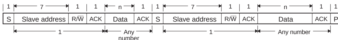
Figure 18-11. I2C Peripheral 7-Bit Addressing Format With Repeated START Condition (FDF = 0, XA = 0 in ICMDR)
