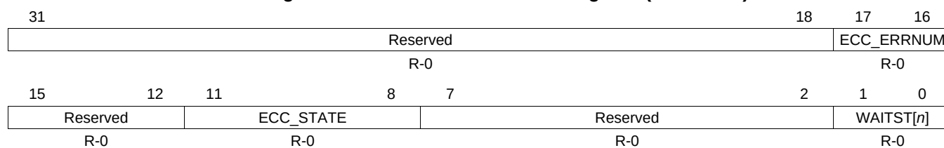
Figure 16-43. NAND Flash Status Register (NANDFSR)
