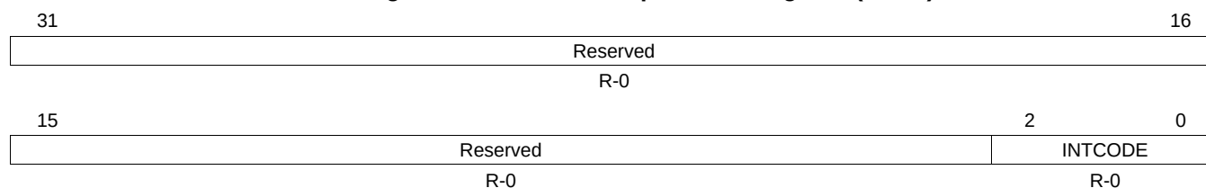
Figure 18-24. I2C Interrupt Vector Register (ICIVR)
