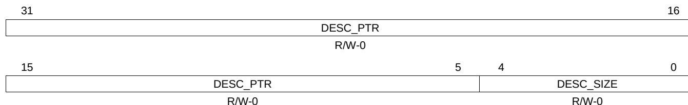
Figure 25-114. Queue Manager Queue N Control Register D (CTRLD[ N ])
