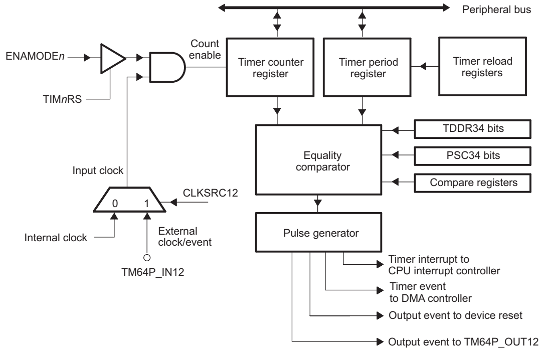
Figure 23-1. Timer Block Diagram
