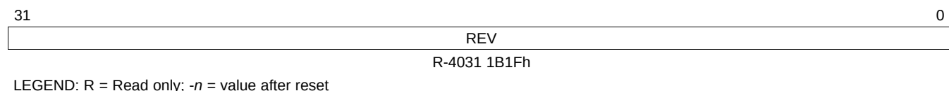
Figure 13-19. Revision ID Register (REVID)
