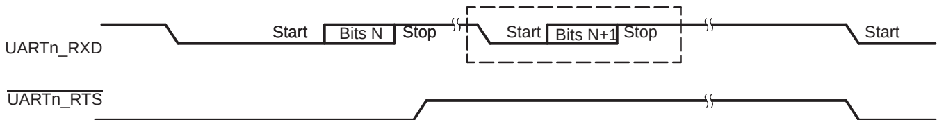
Figure 24-6. Autoflow Functional Timing Waveforms for UARTn_RTS
