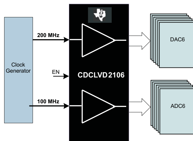
Figure 1. Application Example
