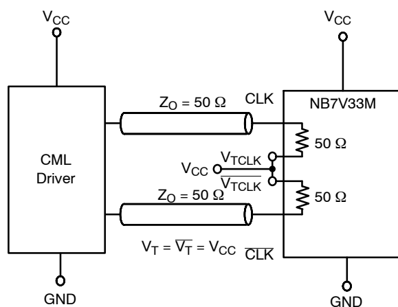
Figure 13. Standard 50 Ω Load CML Interface
