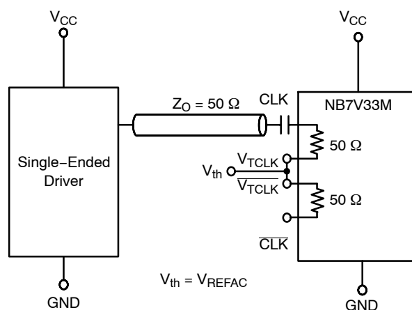
Figure 15. Capacitor-Coupled Single-Ended Interface ( V_{TCLK}/\overline{V_{TCLK}} Connected to V_{REFAC} ; V_{REFAC} Bypassed to Ground with 0.1 μF Capacitor)
