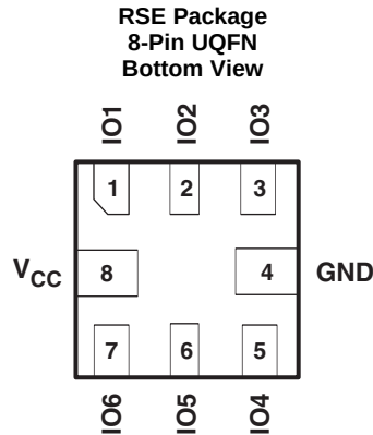
Pin Functions
