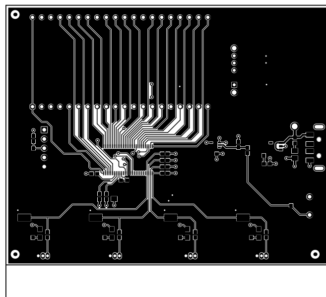
Figure 8. Top Layer
