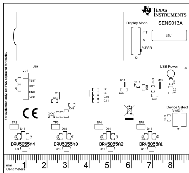
Figure 7. Top Overlay
