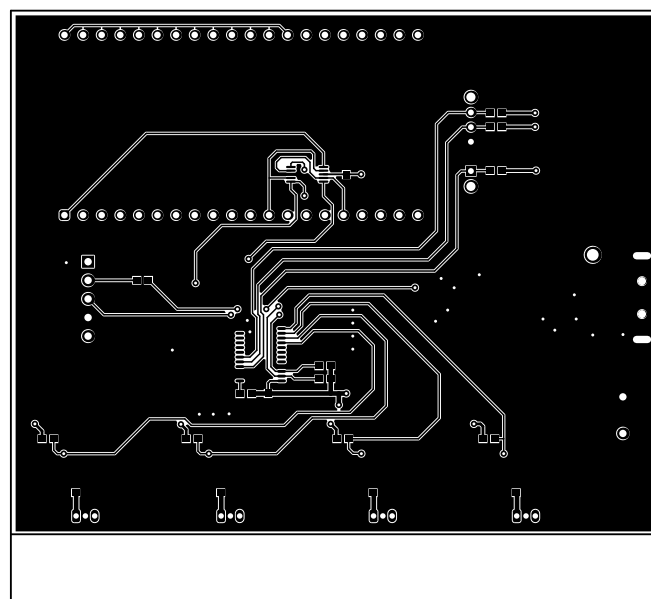
Figure 10. Bottom Layer
