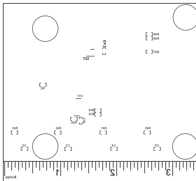
Figure 9. Bottom Overlay
