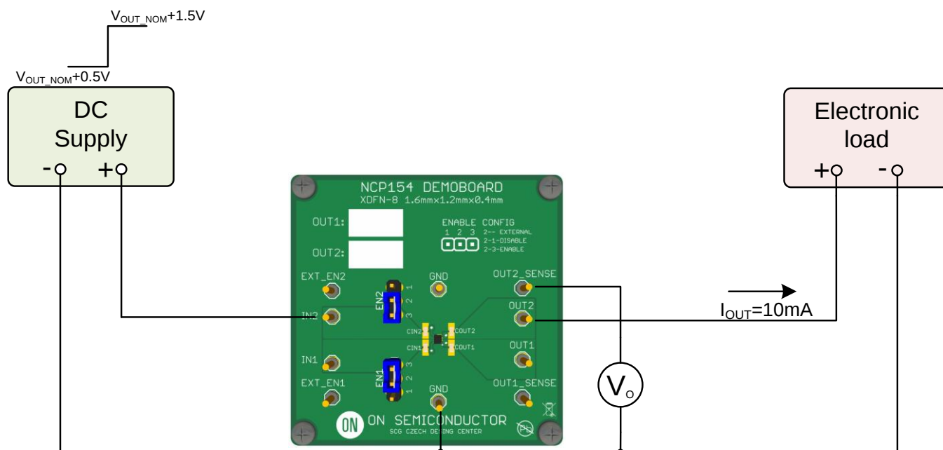
Figure 3: Test configuration for measurement REG_{LINE} , Line Regulation
