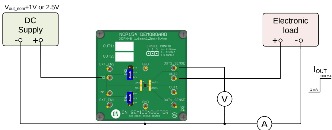
Figure 2: Test configuration for measurement REG LOAD , Load Regulation
