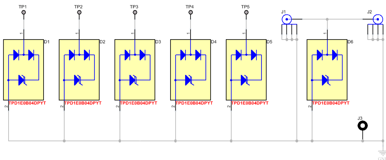
Figure 4. TPD1E0B04DPYEVM Schematic
