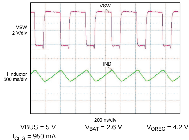
Figure 33. PWM Charging Waveforms
