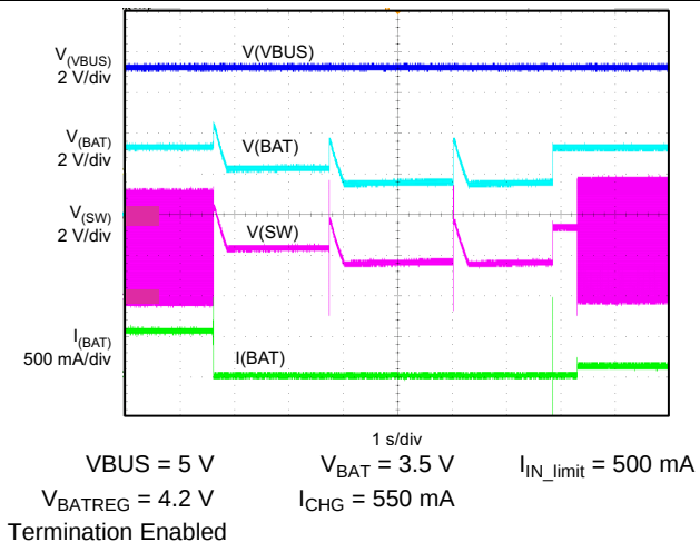
Figure 31. Battery Insertion/Removal Termination Enabled (HOST Mode)
