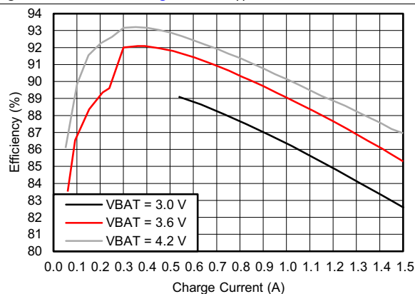
Figure 7. Charger Efficiency
