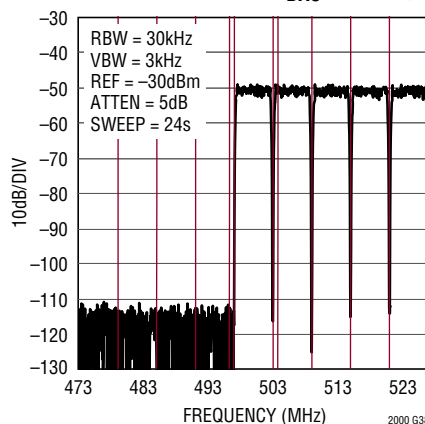
32 Carrier DOCSIS Mid Band Narrowband ACLR, f_{DAC} = 2.5\text{Gsps}
