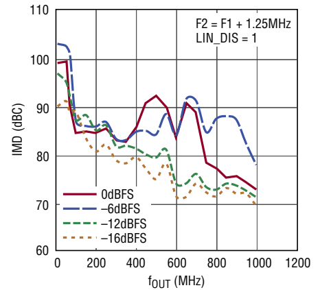
2-Tone IMD vs f_{OUT} and Digital Amplitude, f_{DAC} = 2.5Gsp/s
