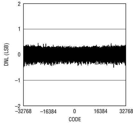
LTC2000-16 Differential Nonlinearity (DNL)
