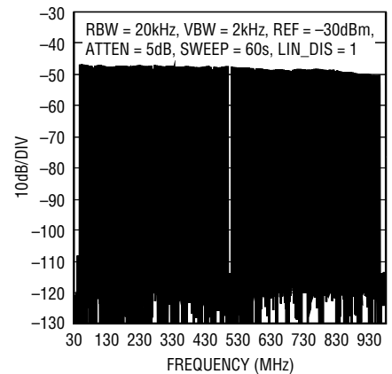
157 Carrier Tones with Gap Channel Wideband ACLR, f_{DAC} = 2.5\text{Gsps}
