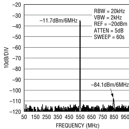
Single Carrier DOCSIS Mid Band Wideband ACLR, f_{DAC} = 2.5\text{Gsps}
