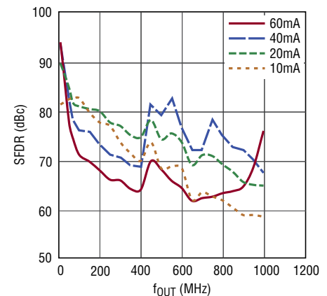
SFDR vs f_{OUT} and I_{OUTFS} , f_{DAC} = 2.5\text{Gsps}
