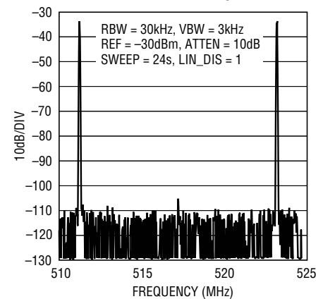
157 Carrier Tones with Gap Channel Narrowband ACLR, f_{DAC} = 2.5\text{Gsps}
