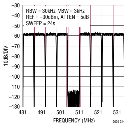
157 Carrier DOCSIS Gap Channel Narrowband ACLR, f_{DAC} = 2.5\text{Gsps}
