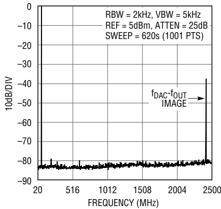
Single-Tone Spectrum at f_{OUT} = 70\text{MHz} , f_{DAC} = 2.5\text{Gsps}
