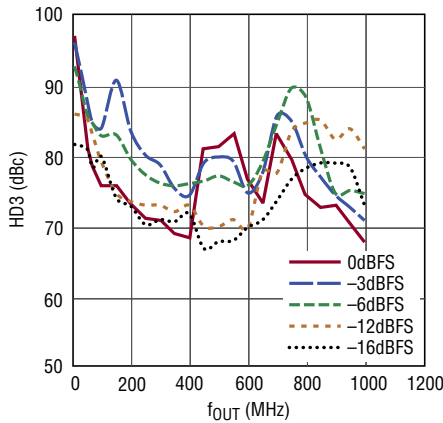
HD3 vs f_{OUT} and Digital Amplitude (dBFS), f_{DAC} = 2.5Gsp/s
