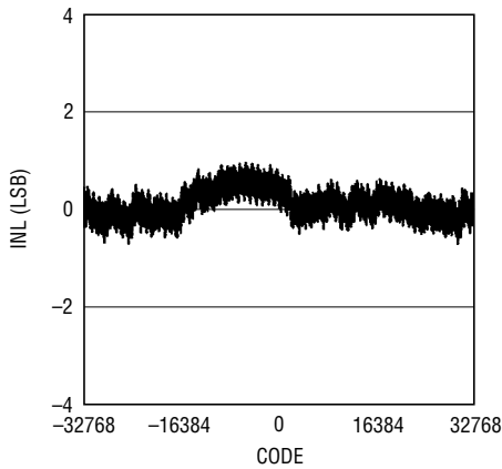
LTC2000-16 Integral Nonlinearity (INL)
