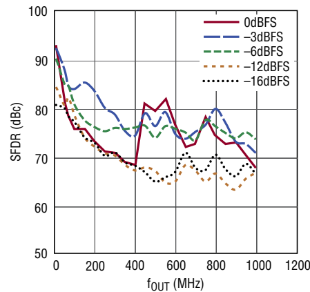
SFDR vs f_{OUT} and Digital Amplitude (dBFS), f_{DAC} = 2.5\text{Gsps}
