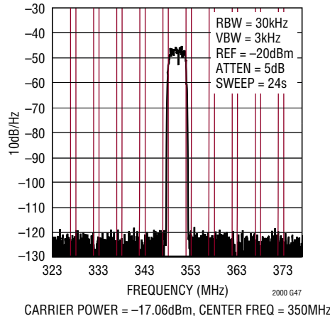
LTC2000-16 Single Carrier WCDMA ACLR at 350MHz, f_{DAC} = 2.5Gps
