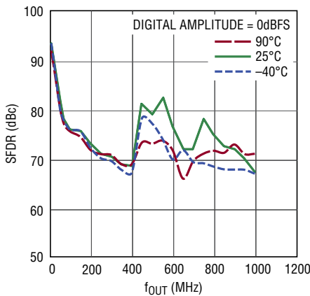
SFDR vs f_{OUT} and Temperature, f_{DAC} = 2.5\text{Gsps}
