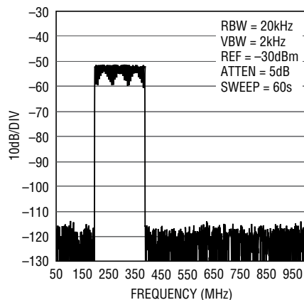
32-Carrier DOCSIS Low Band Wideband ACLR, f_{DAC} = 2.5\text{Gsps}
