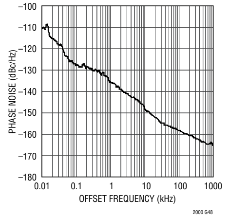
Additive Phase Noise, f_{OUT} = 65MHz , f_{DAC} = 2.5Gps
