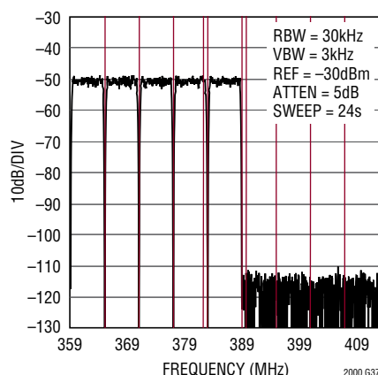
32-Carrier DOCSIS Low Band Narrowband ACLR, f_{DAC} = 2.5\text{Gsps}
