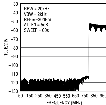
32 Carrier DOCSIS High Band Wideband ACLR, f_{DAC} = 2.5\text{Gsps}
