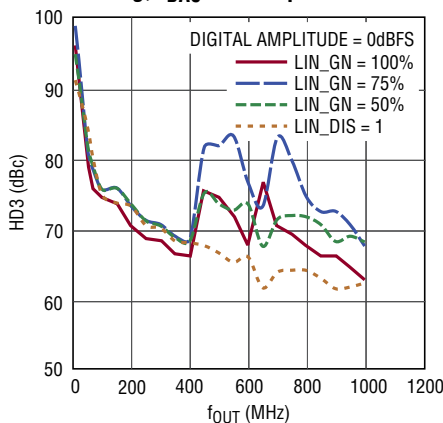
HD3 vs f_{OUT} and Linearization Setting, f_{DAC} = 2.5Gsp/s
