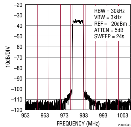
Single Carrier DOCSIS High Band Narrowband ACLR, f_{DAC} = 2.5\text{Gsps}
