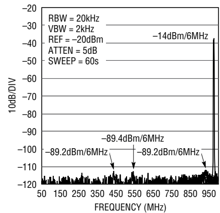
Single Carrier DOCSIS High Band Wideband ACLR, f_{DAC} = 2.5\text{Gsps}
