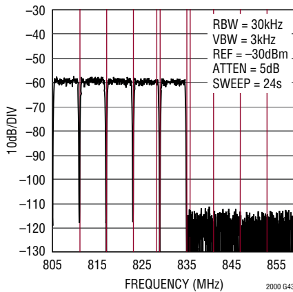
128 Carrier DOCSIS Low Band Narrowband ACLR, f_{DAC} = 2.5\text{Gsps}
