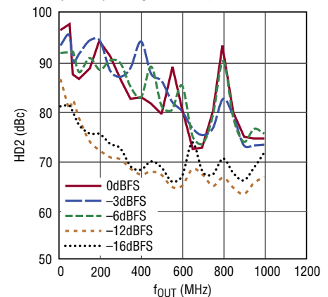
HD2 vs f_{OUT} and Digital Amplitude (dBFS), f_{DAC} = 2.5\text{Gsps}
