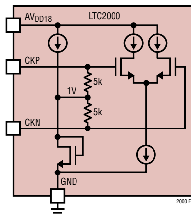
Figure 11. DAC Sample Clock Receiver
