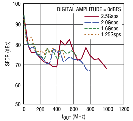
SFDR vs f_{OUT} and f_{DAC}
