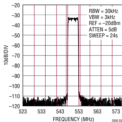
Single Carrier DOCSIS Mid Band Narrowband ACLR, f_{DAC} = 2.5\text{Gsps}
