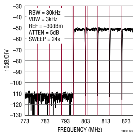
32 Carrier DOCSIS High Band Narrowband ACLR, f_{DAC} = 2.5\text{Gsps}
