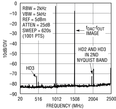
Single-Tone Spectrum at f_{OUT} = 990\text{MHz} , f_{DAC} = 2.5\text{Gsps}
