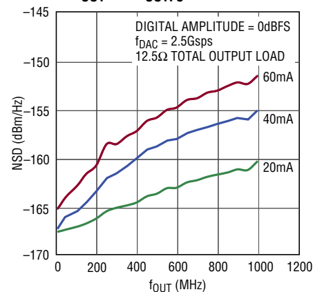
LTC2000-16 Single-Tone NSD vs f_{OUT} and I_{OUTFS}
