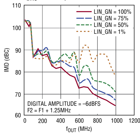
2-Tone IMD vs f_{OUT} and Linearization Setting, f_{DAC} = 2.5Gsp/s
