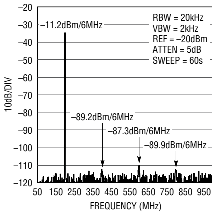
Single Carrier DOCSIS Low Band Wideband ACLR, f_{DAC} = 2.5\text{Gsps}
