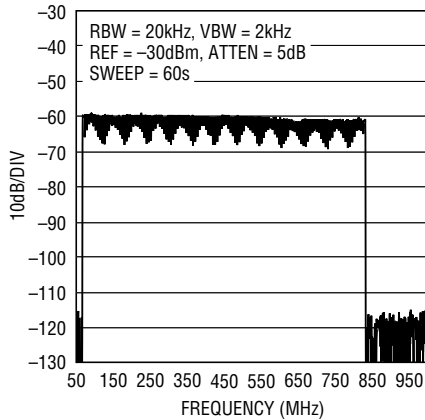
128 Carrier DOCSIS Low Band Wideband ACLR, f_{DAC} = 2.5\text{Gsps}
