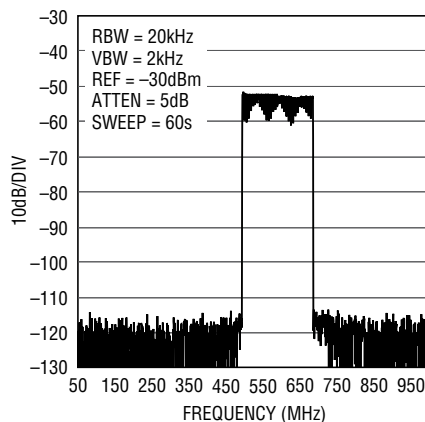
32-Carrier DOCSIS Mid Band Wideband ACLR, f_{DAC} = 2.5\text{Gsps}
