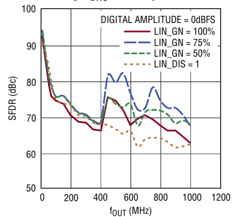
SFDR vs f_{OUT} and Linearization Setting, f_{DAC} = 2.5Gsp/s
