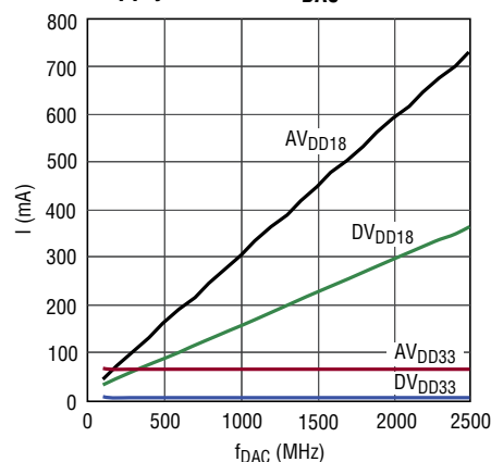
Supply Current vs f_{DAC}
