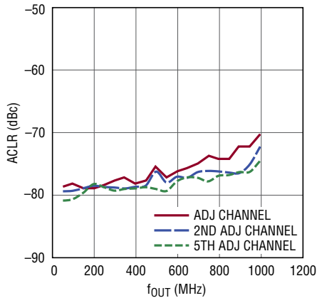
LTC2000-16 Single Carrier WCDMA ACLR vs f_{OUT} , f_{DAC} = 2.5Gps
