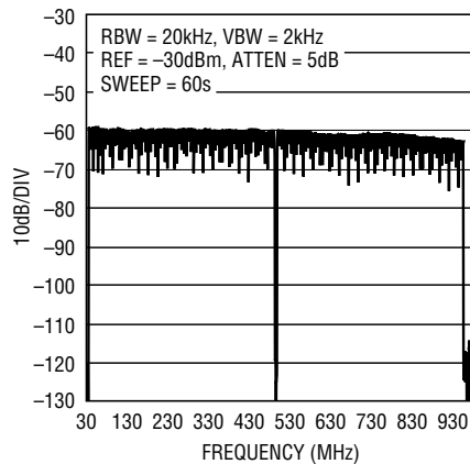
157 Carrier DOCSIS Gap Channel Wideband ACLR, f_{DAC} = 2.5\text{Gsps}
