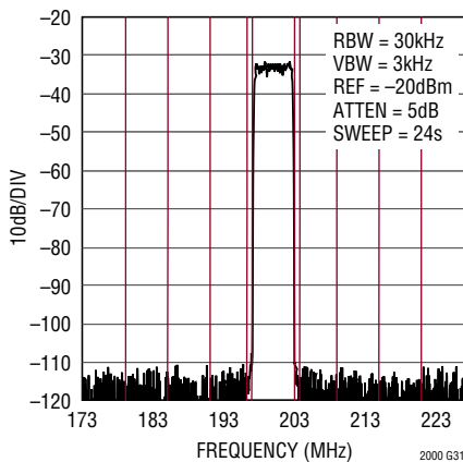
Single Carrier DOCSIS Low Band Narrowband ACLR, f_{DAC} = 2.5\text{Gsps}
