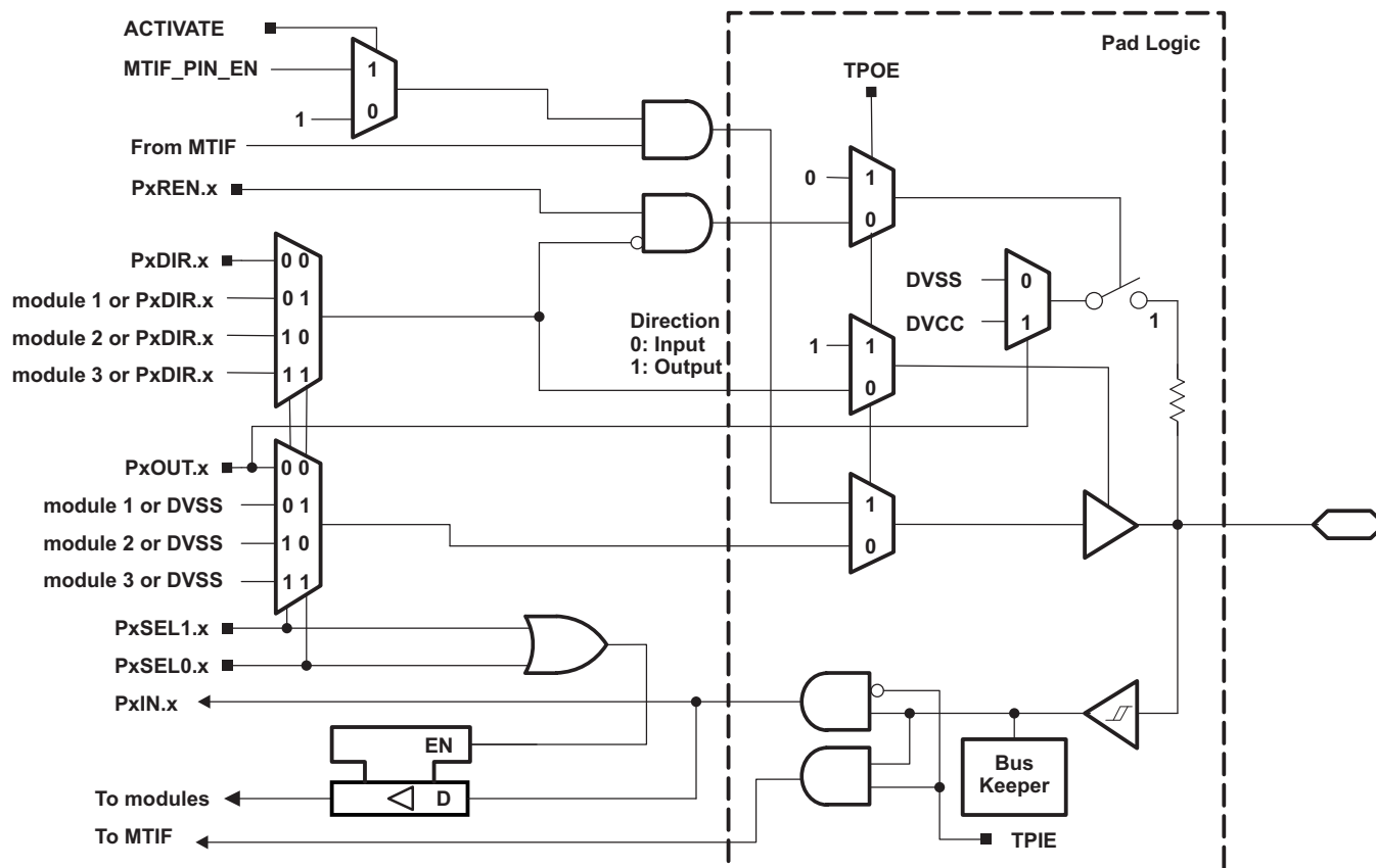
Figure 6-14. Port P7 (P7.4) Diagram
