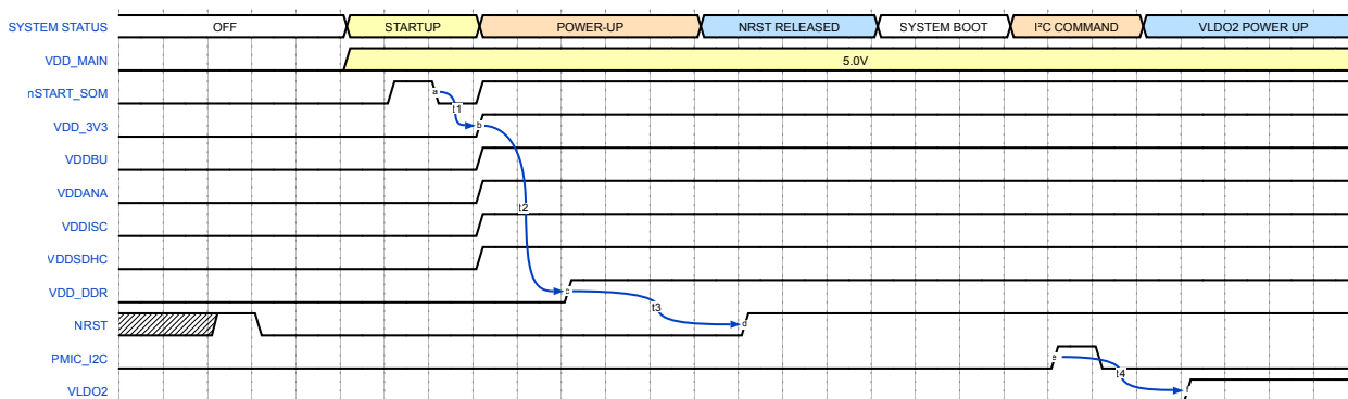
Figure 4-9. ATSAM5D27-WLSOM1 Single Supply Connection: Power-On Sequence
