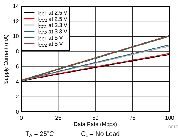
Figure 12. ISO7763-Q1 Supply Current vs Data Rate (With No Load)
