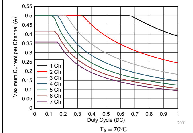
Figure 9. D Package Maximum Collector Current vs Duty Cycle
