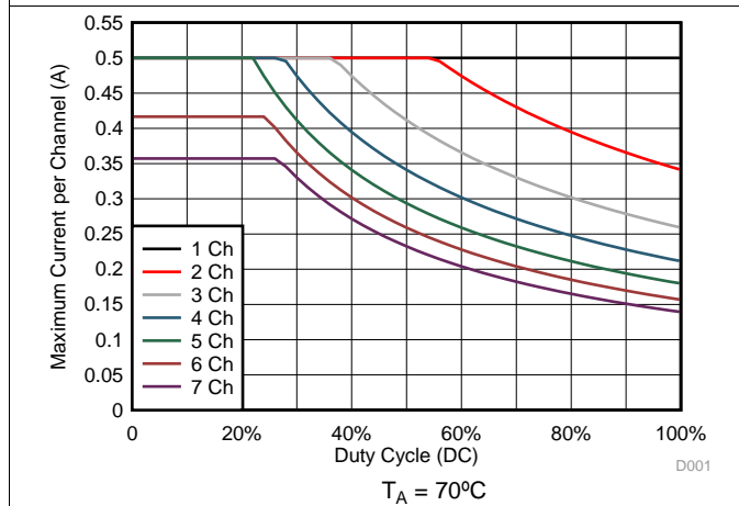
Figure 11. N Package Maximum Collector Current vs Duty Cycle
