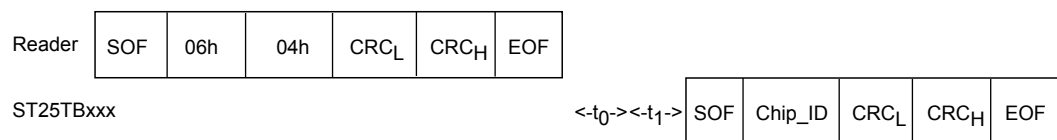
Figure 48. Pcall16 frame exchange between reader and ST25TB04K
