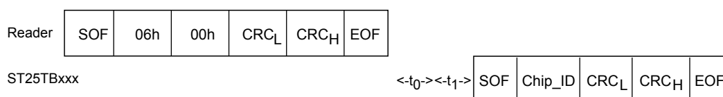
Figure 20. Initiate frame exchange between reader and ST25TB04K
