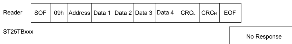
Figure 41. Write_block frame exchange between reader and ST25TB04K
