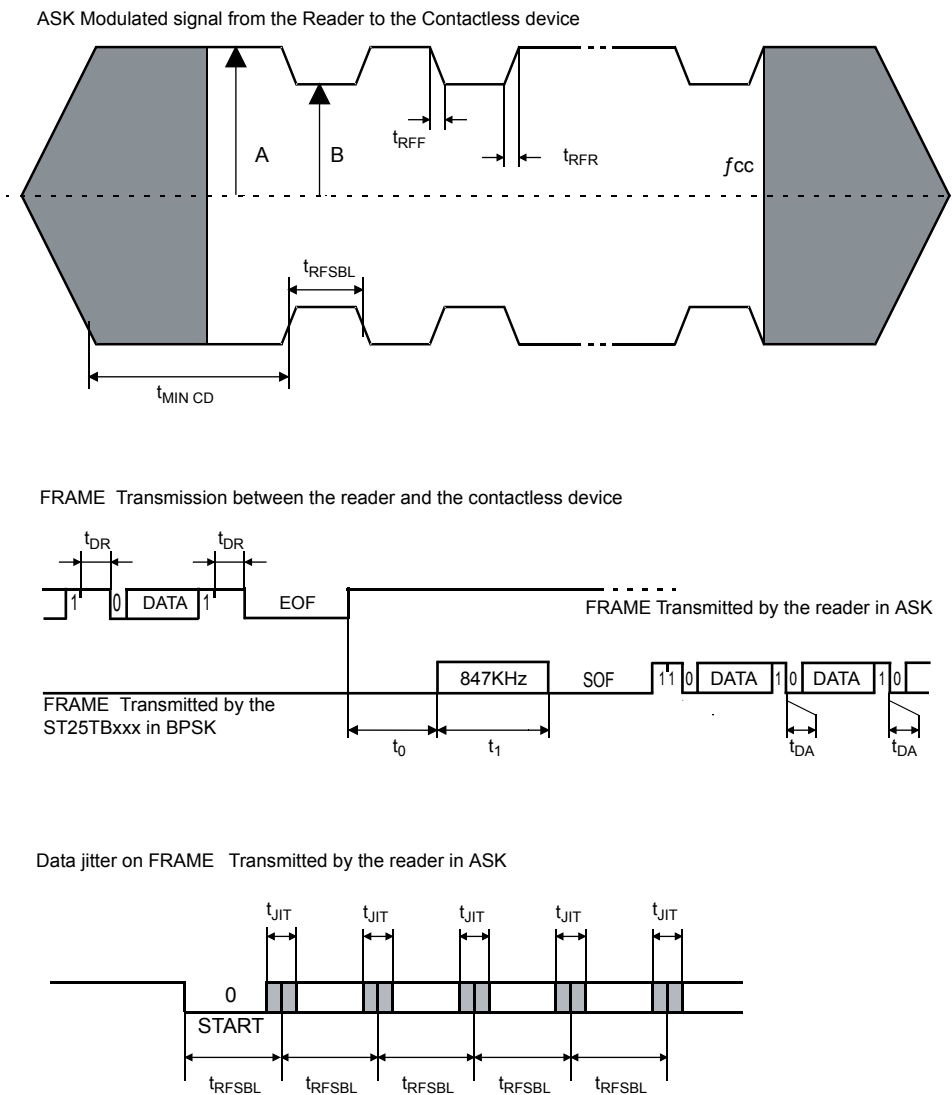
Figure 46. ST25TB04K synchronous timing, transmit and receive
