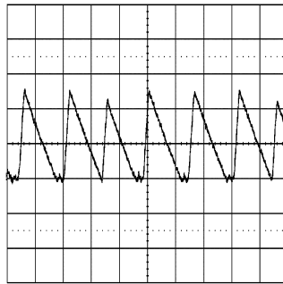
Figure 36. Transition Mode Operation V_{IN} = 24 \text{ V} , V_O = 3.3 \text{ V} , I_O = 0.35 \text{ A} 2 \mu\text{s/div}
