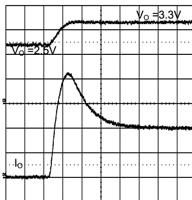
Figure 33. Prebiased Start-Up
