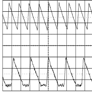
Figure 35. CCM and DCM Operating Modes V_{IN} = 24 \text{ V} , V_O = 3.3 \text{ V} , I_O = 2 \text{ A} / 0.32 \text{ A} 2 \mu\text{s/div}
