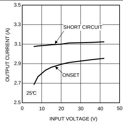
Figure 30. Current Limit 3.3\text{-}V_{OUT} at 25^\circ\text{C}
