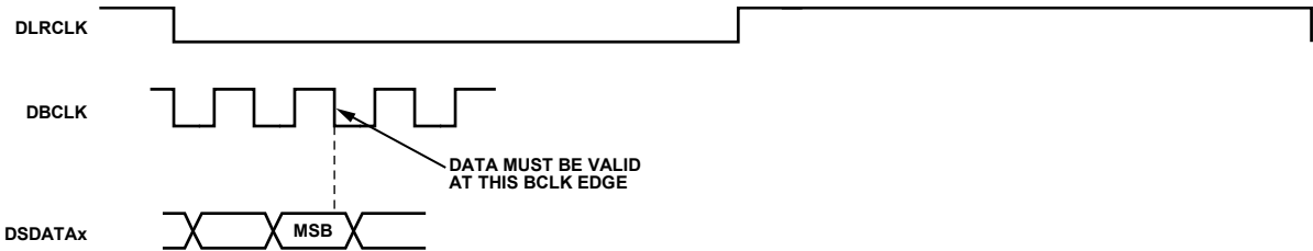
Figure 21. Inverted Bit Clock Mode in DAC Serial Data Transmission (Applicable in Stereo and TDM, Useful for High Frequency TDM Transmission)
