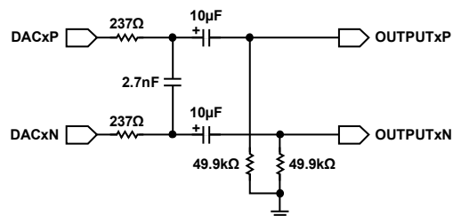
Figure 9. Typical DAC Output Passive Filter Circuit (Differential)
