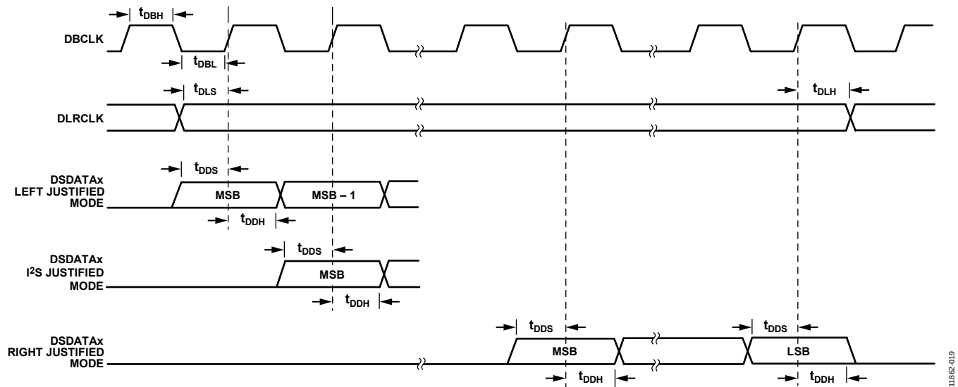
Figure 19. DAC Serial Timing
