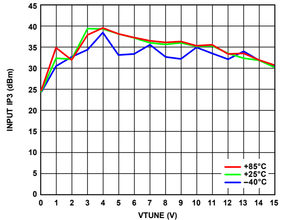
Figure 41. Input IP3 vs. VTUNE at Various Temperatures, Input Power ( P_{IN} ) = 20 dBm
