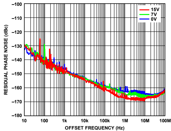
Figure 42. Residual Phase Noise vs. Offset Frequency at Various VTUNE
