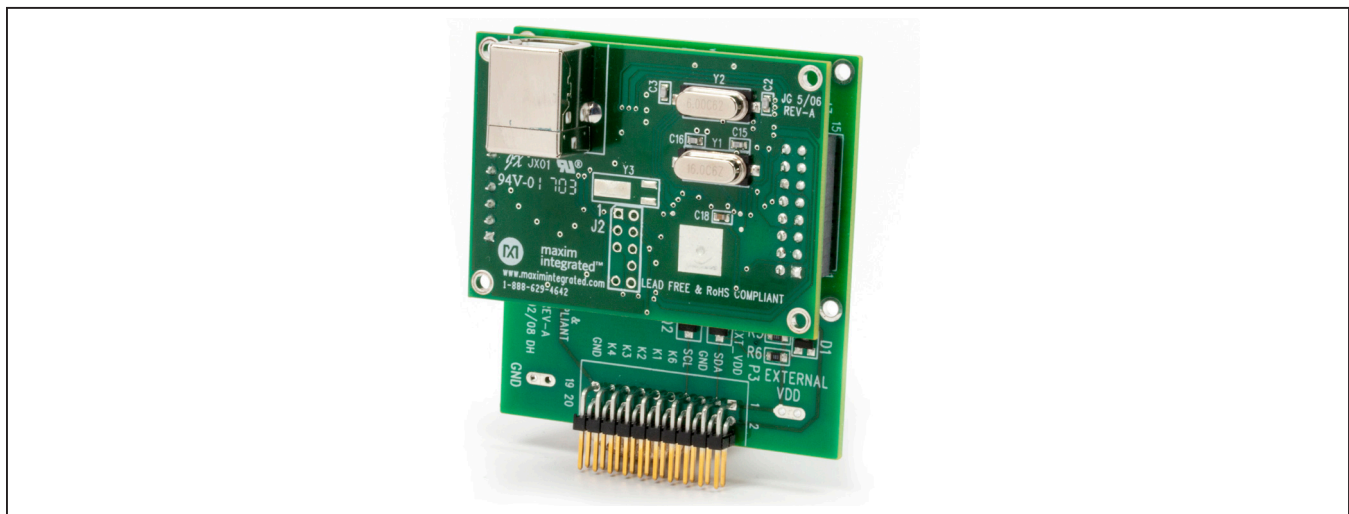
Figure 2. MINIQUSB Board
