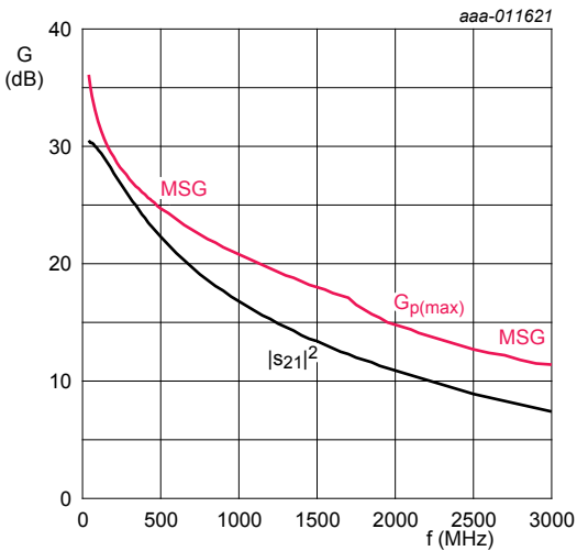
I_C = 15\text{ mA} ; V_{CE} = 8\text{ V} ; T_{amb} = 25^\circ\text{C} . Figure 10. Gain as a function of frequency; typical values
