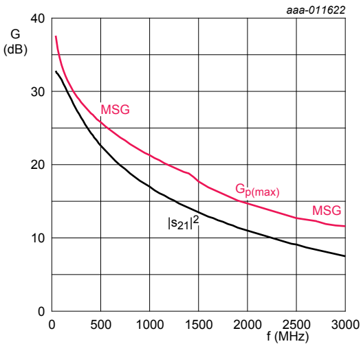
I_C = 25\text{ mA} ; V_{CE} = 8\text{ V} ; T_{amb} = 25^\circ\text{C} . Figure 11. Gain as a function of frequency; typical values
