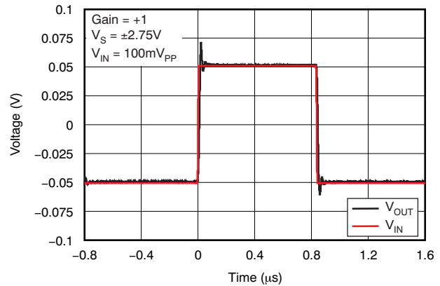
Figure 26. Small-Signal Step Response
