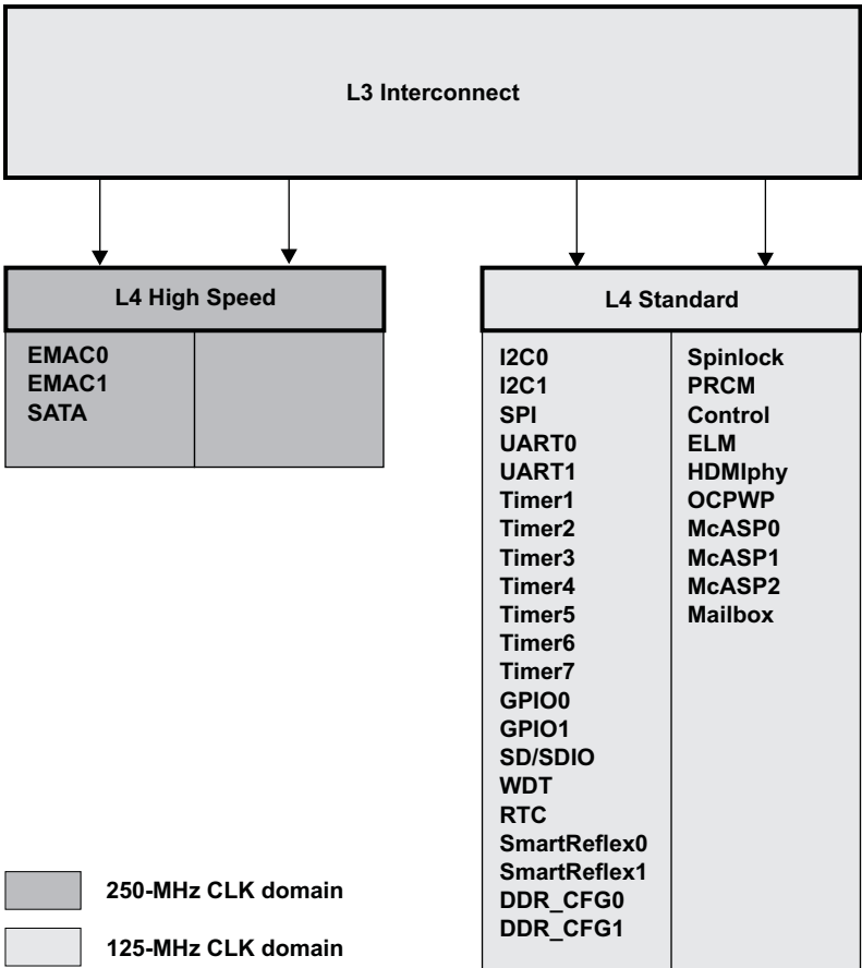
Figure 7-2. L4 Architecture
