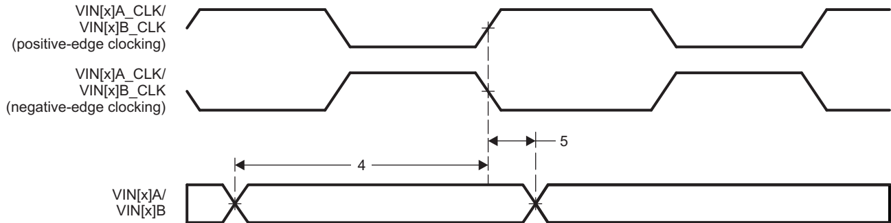
Figure 9-69. HDVPSS Input Timing
