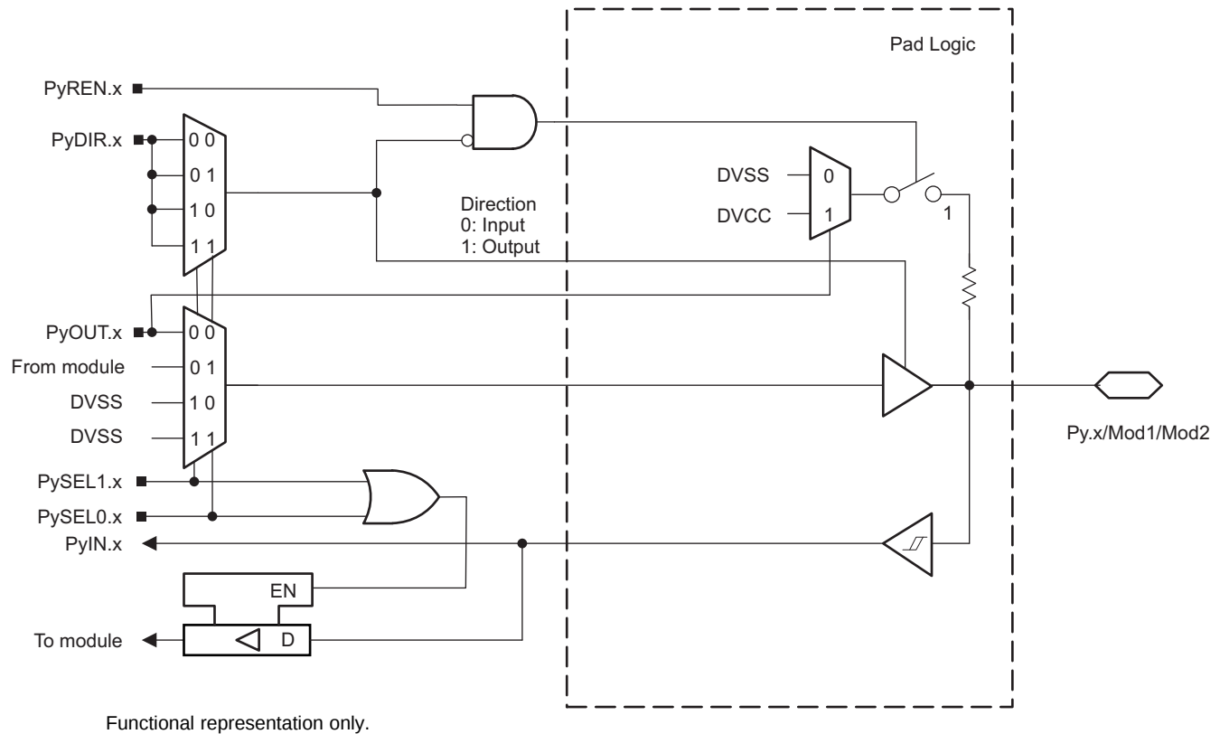
Figure 6-11. P7.3 Pin Schematic
