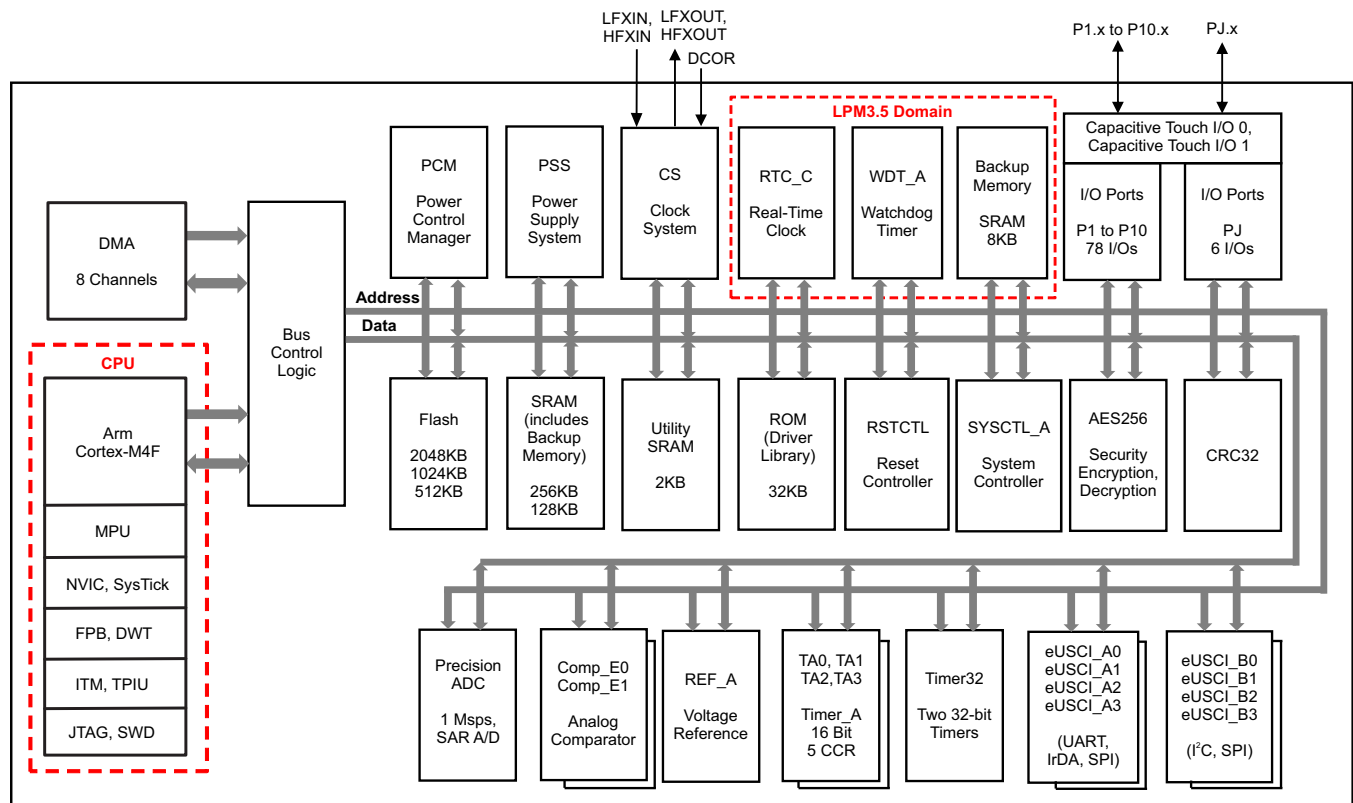
Figure 1-2. MSP432P401xT Functional Block Diagram
