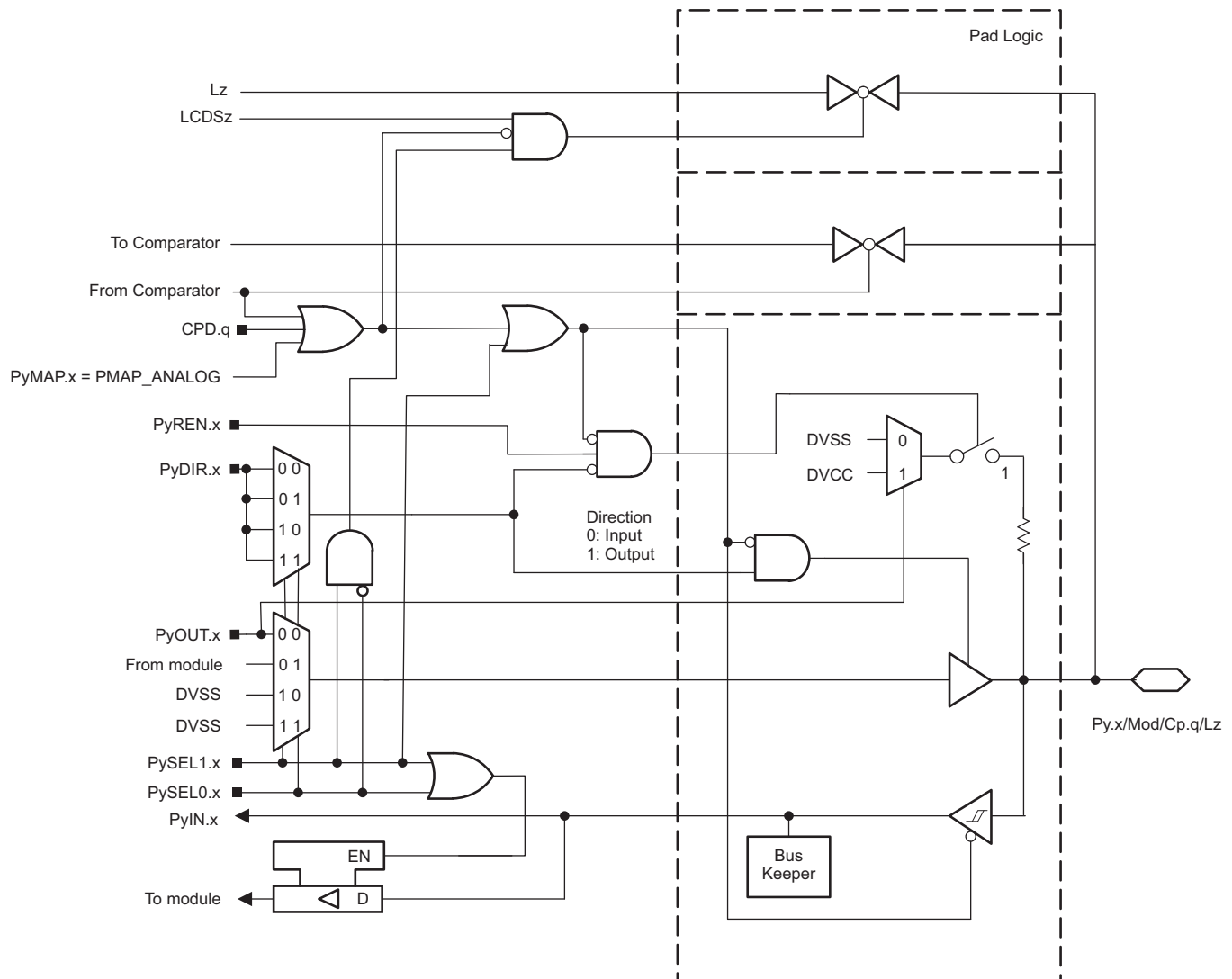
Figure 6-19. Py.x/Mod/Cp.q/Lz Pin Schematic
