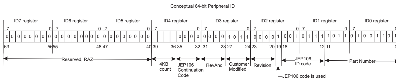
Figure 6-25. ROM PID Entries for MSP432P4x1xT Device
