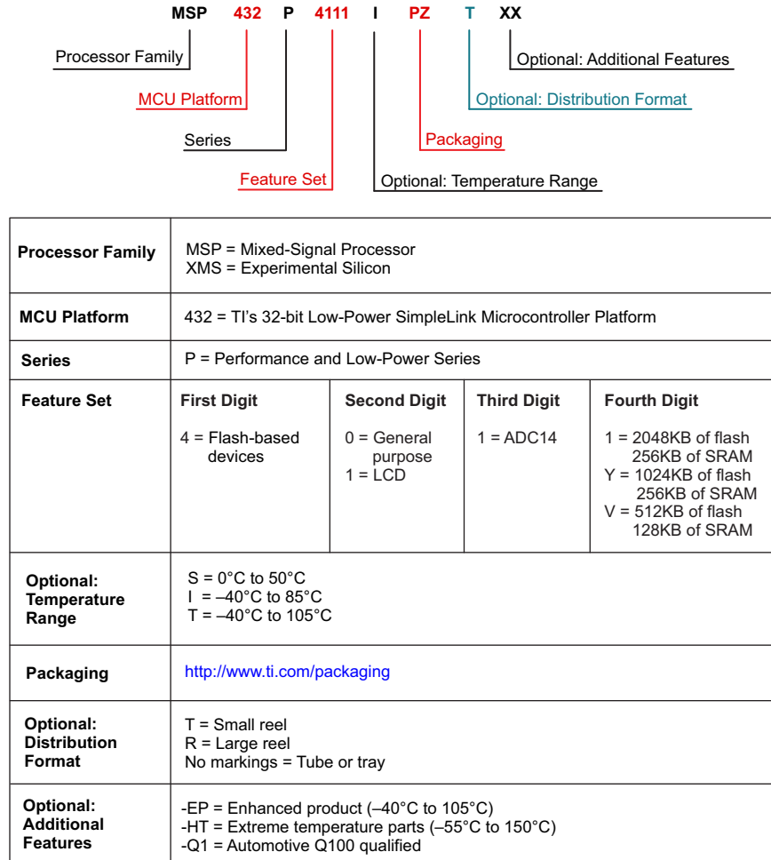
Figure 8-1. Device Nomenclature
