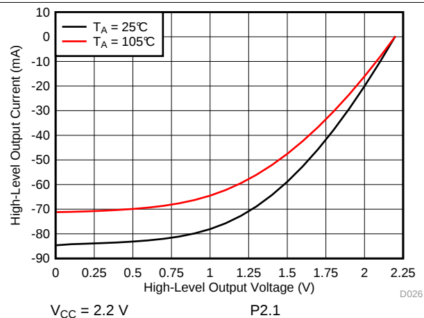
Figure 5-25. High-Level Output Voltage vs High-Level Output Current
