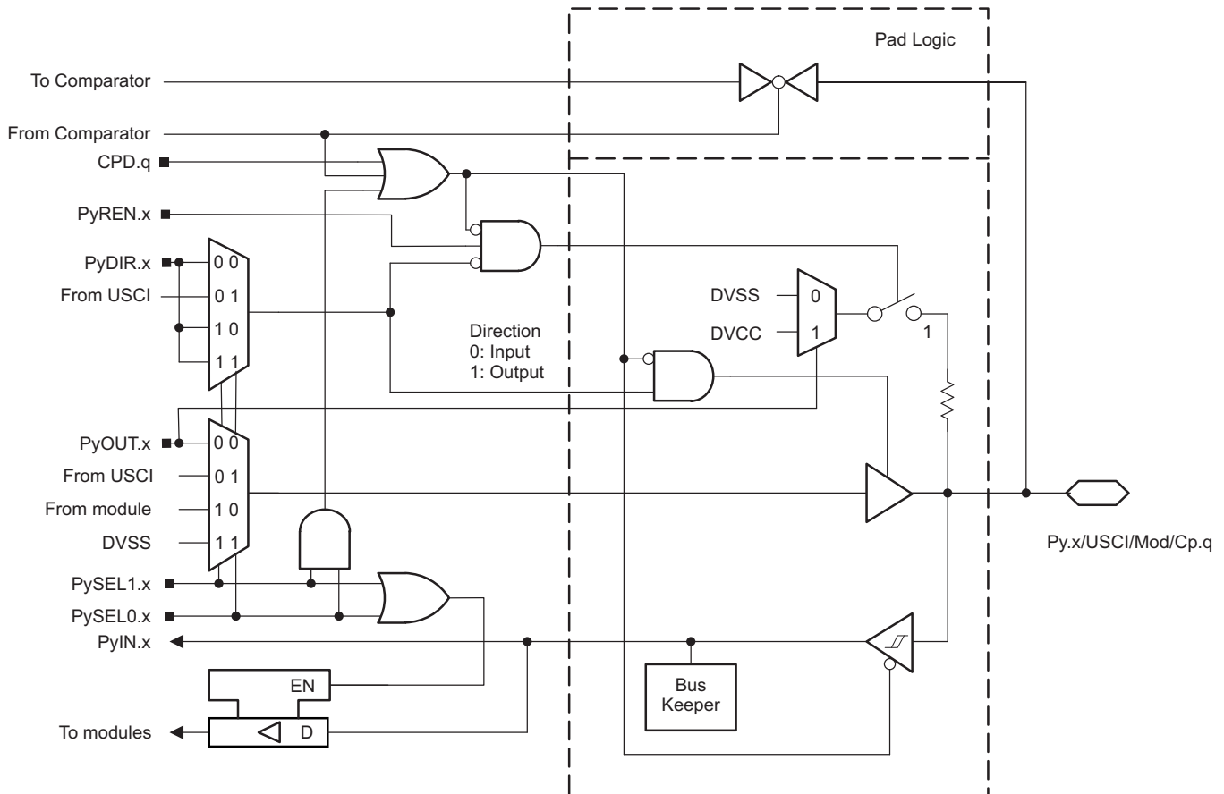
Figure 6-17. Py.x/USCI/Mod/Cp.q Pin Schematic
