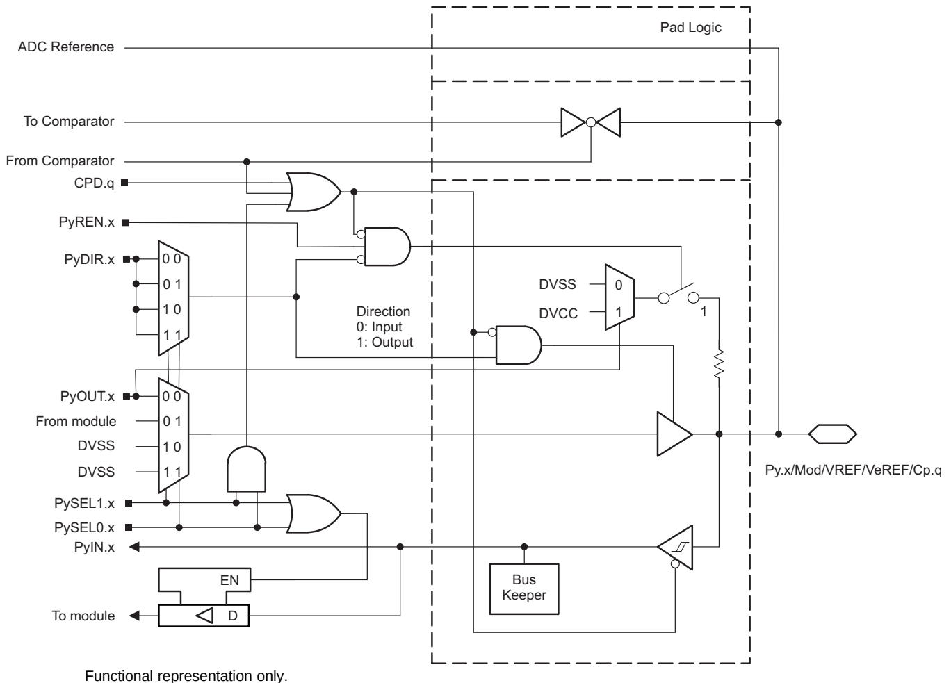
Figure 6-14. Py.x/Mod/VREF/VeREF/Cp.q Pin Schematic
