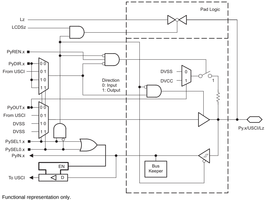
Figure 6-8. Py.x/USCI/Lz Pin Schematic
