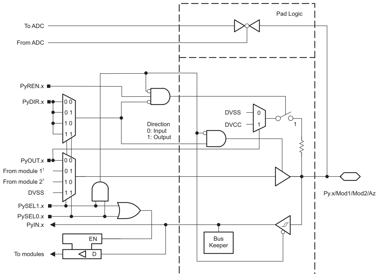
Figure 6-12. Py.x/Mod1/Mod2/Az Pin Schematic
