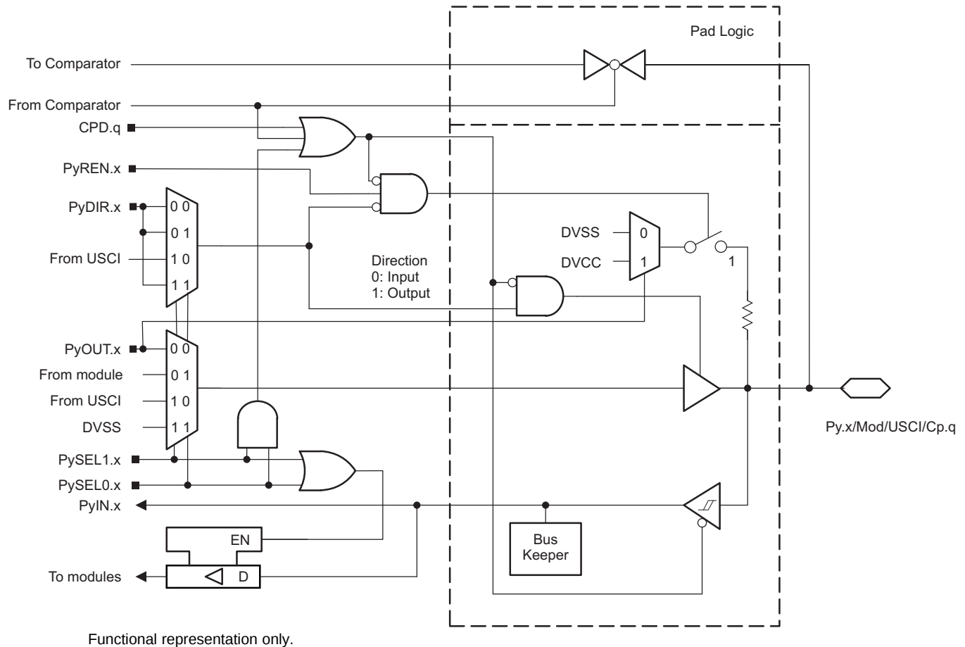
Figure 6-16. Py.x/Mod/USCI/Cp.q Pin Schematic
