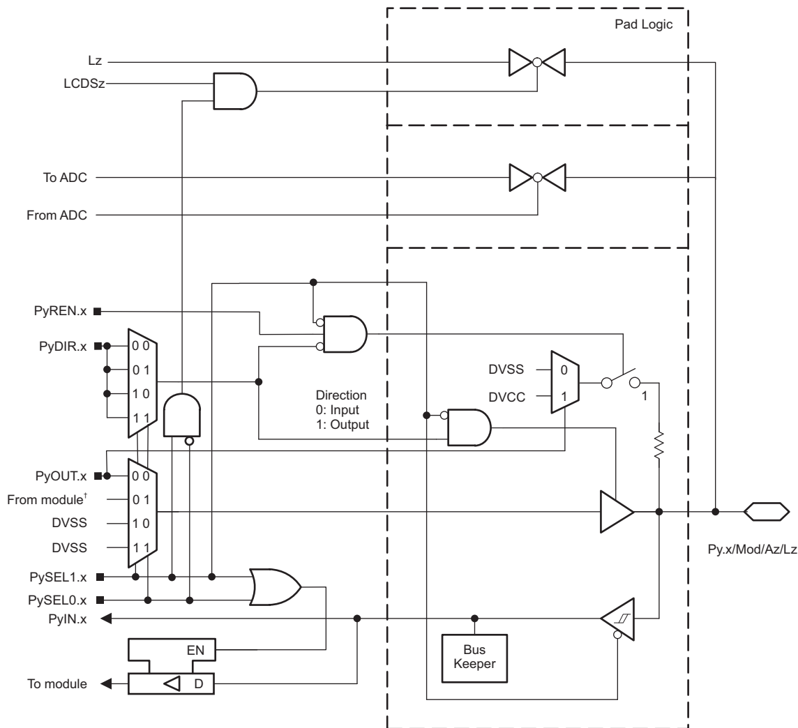
Figure 6-13. Py.x/Mod/Az/Lz Pin Schematic
