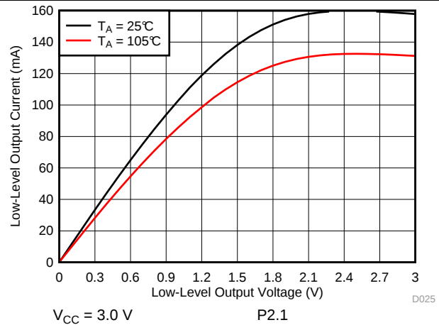
Figure 5-24. Low-Level Output Voltage vs Low-Level Output Current
