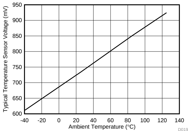
Figure 5-29. Typical Temperature Sensor Voltage
