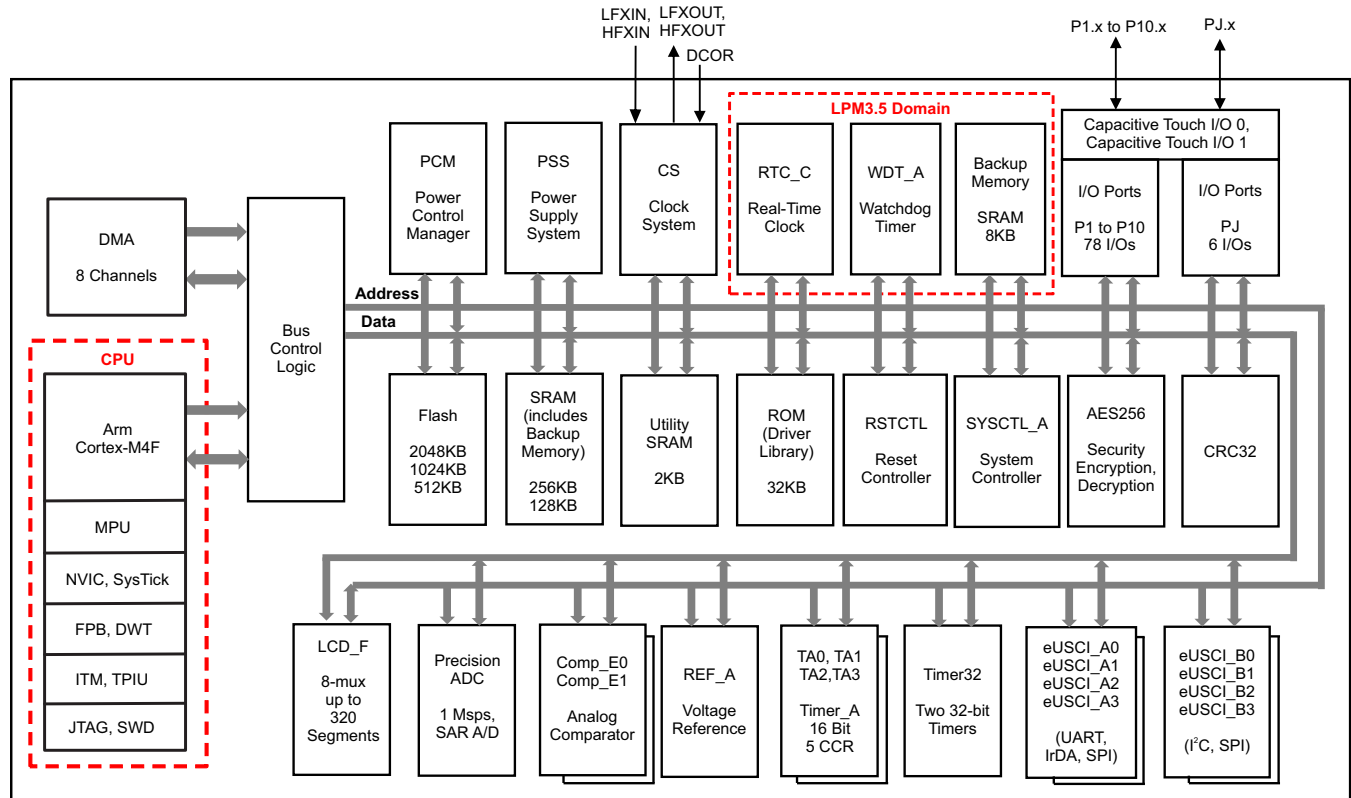
Figure 1-1. MSP432P411xT Functional Block Diagram
