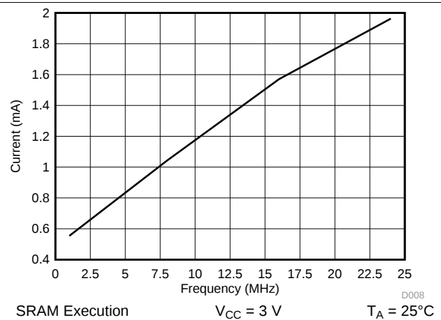
Figure 5-8. Frequency vs Current Consumption
