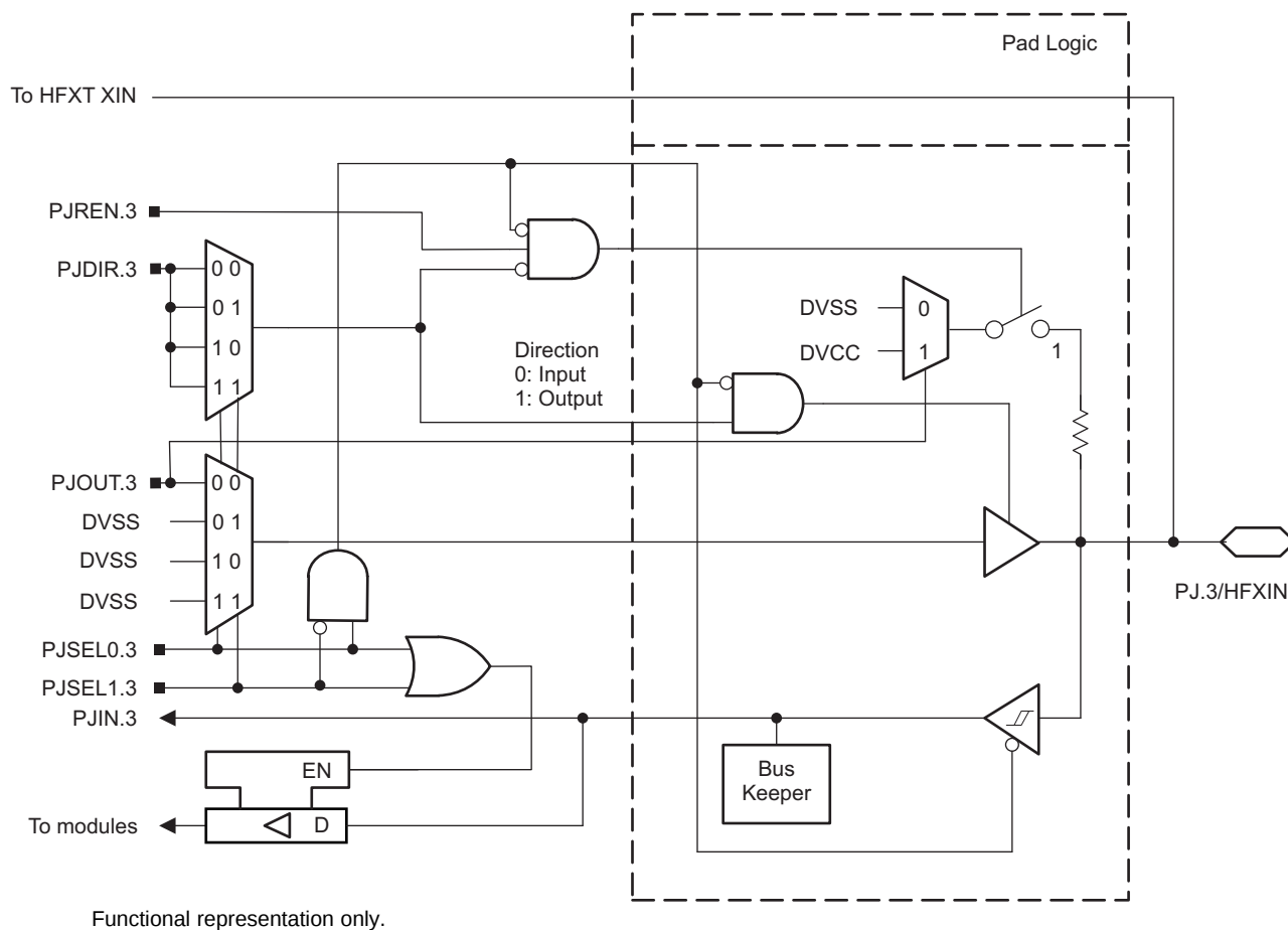
Figure 6-23. Port PJ (PJ.3) Schematic
