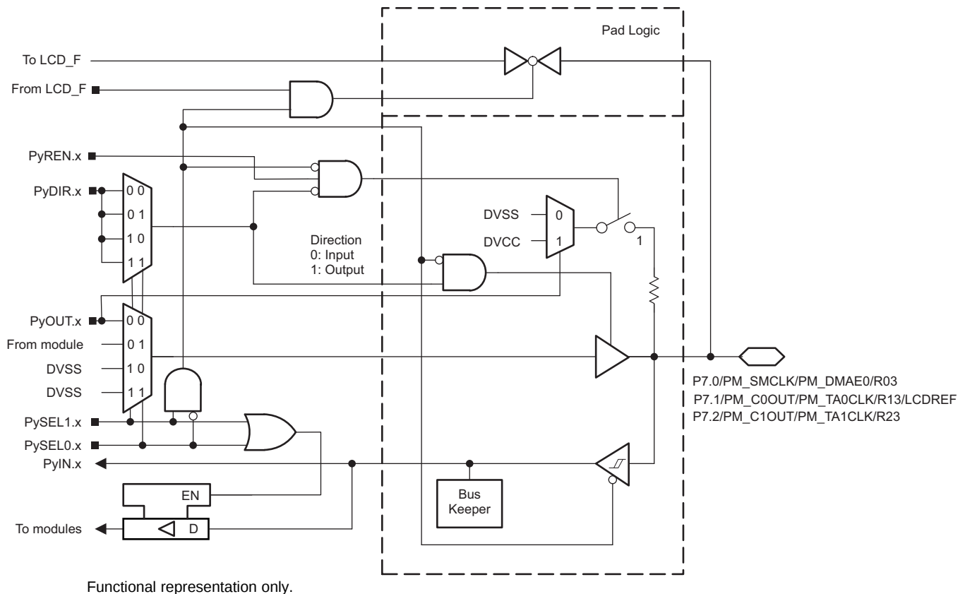
Figure 6-10. P7.0, P7.1 and P7.2 Pin Schematic
