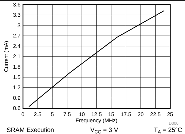
Figure 5-6. Frequency vs Current Consumption
