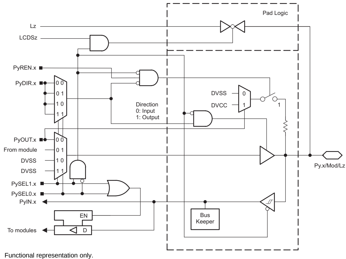
Figure 6-9. Py.x/Mod/Lz Pin Schematic
