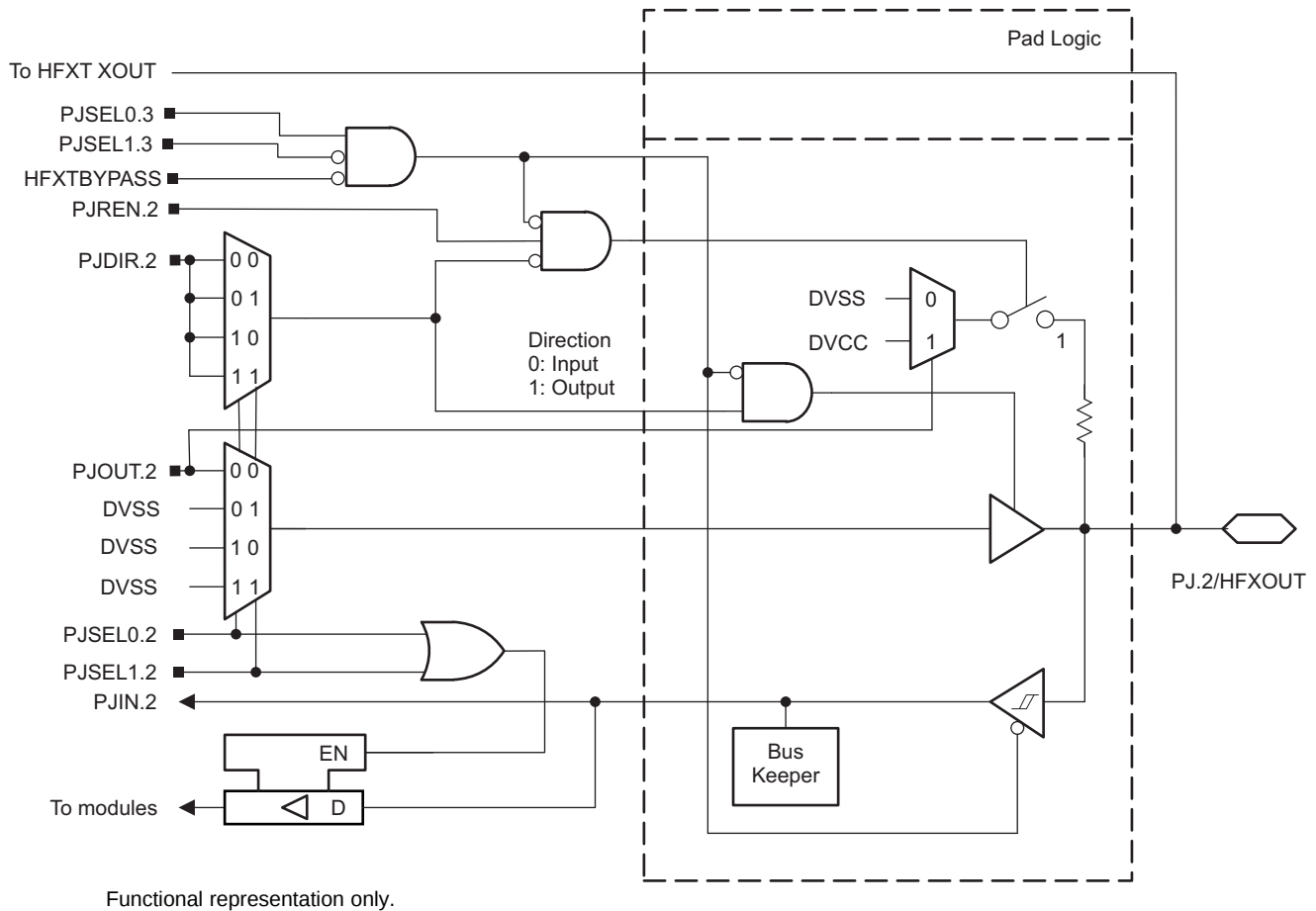
Figure 6-22. Port PJ (PJ.2) Schematic
