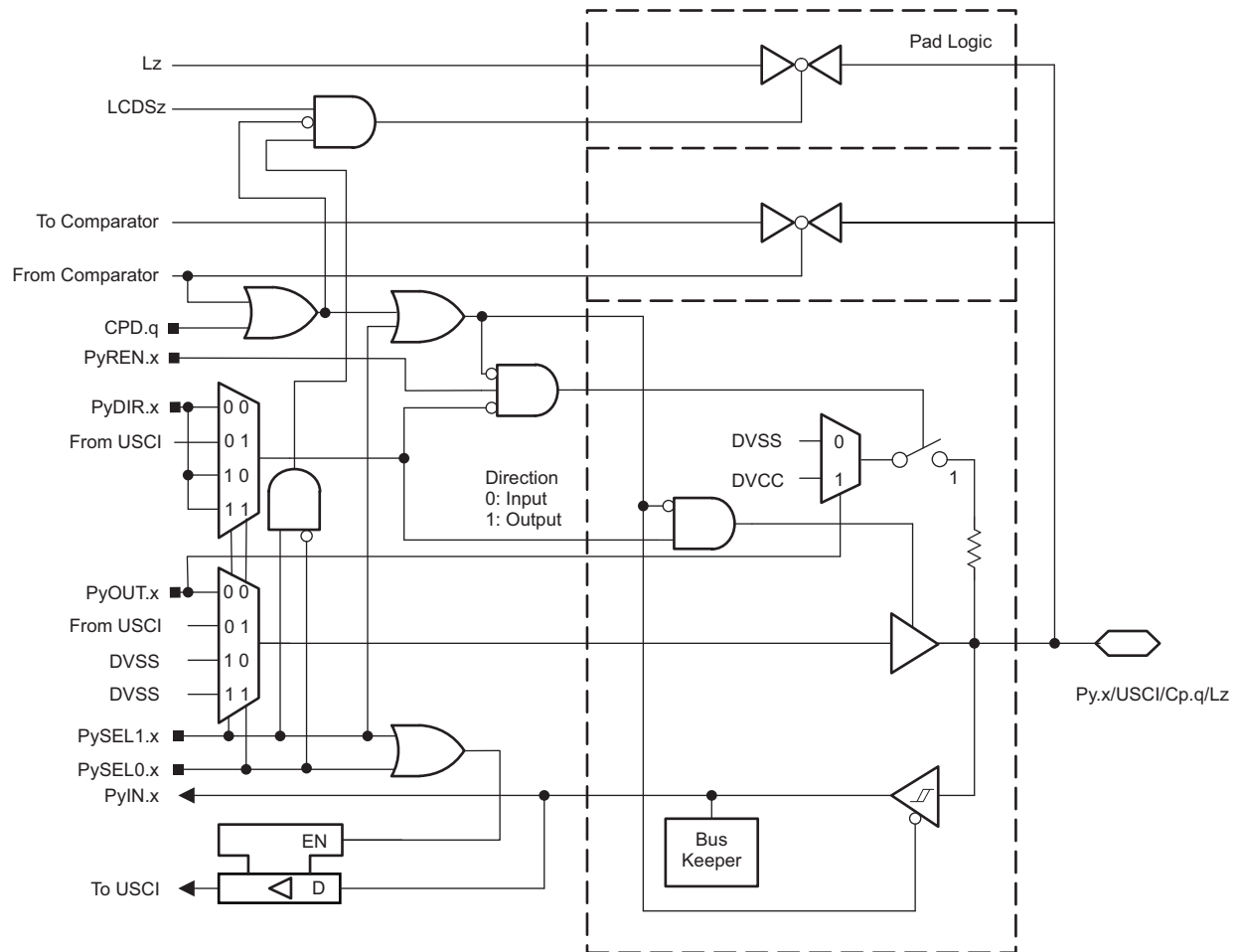
Figure 6-15. Py.x/USCI/Cp.q Pin Schematic
