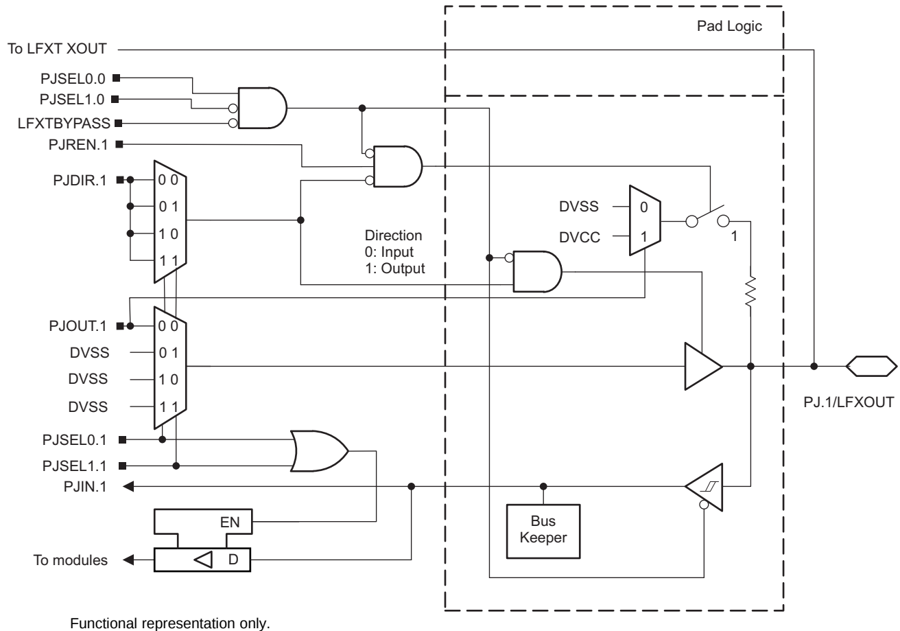
Figure 6-21. Port PJ (PJ.1) Schematic
