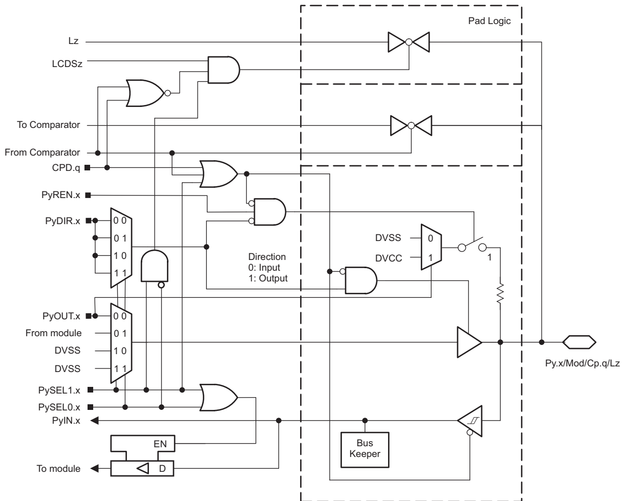
Figure 6-18. Py.x/Mod/Cp.q/Lz Pin Schematic
