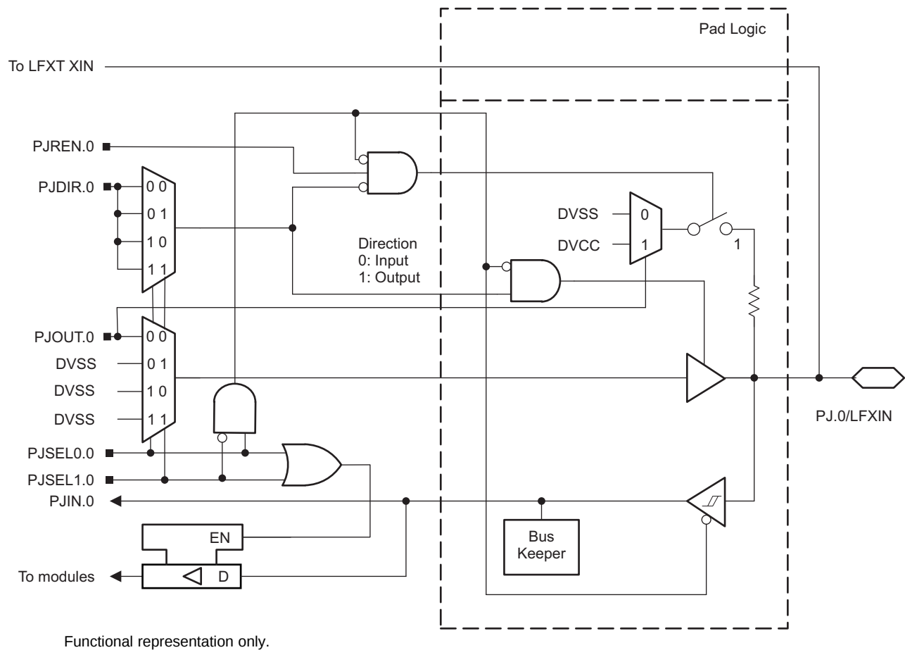
Figure 6-20. Port PJ (PJ.0) Schematic
