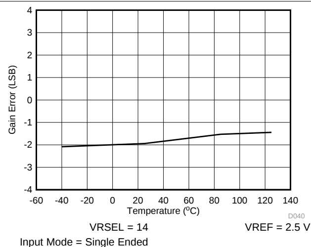
Figure 5-67. Gain Error vs Temperature
