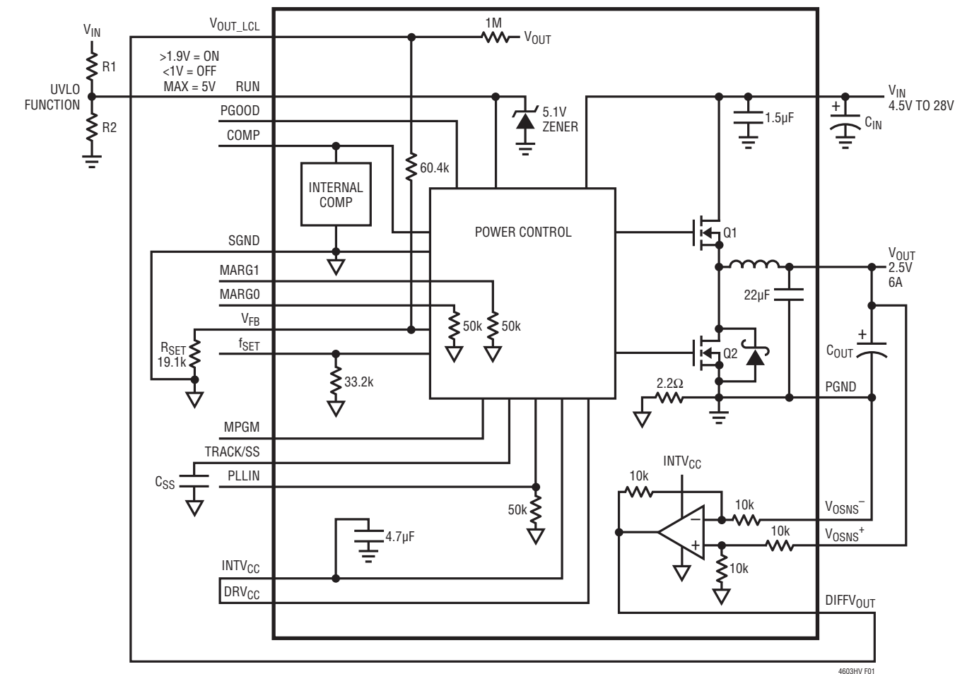
Figure 1. Simplified LTM4603HV Block Diagram
