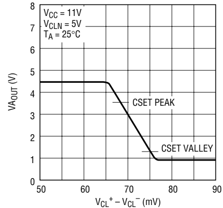
Current Limit Amplifier CA1 Gain at V_{CC} = 11V , V_{CL}^- = 5V
