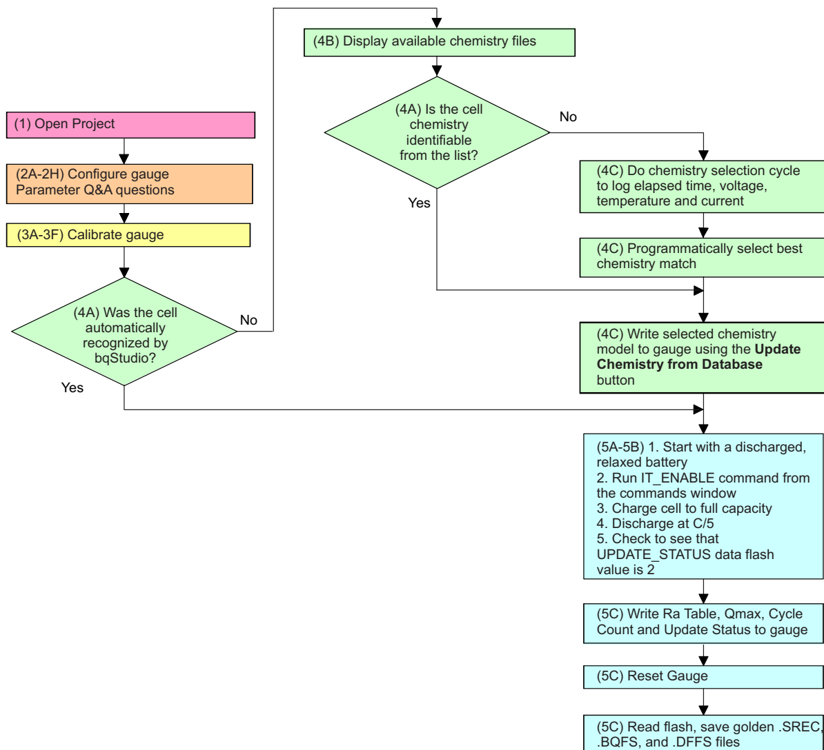
Figure 15. bqStudio Flowchart
