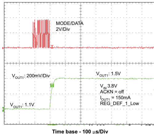
Figure 34. V_{OUT1} Change With EasyScale™ Interface
