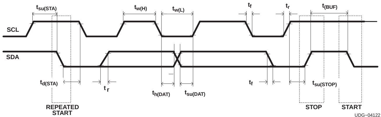
Figure 2. I²C Timing Diagram
