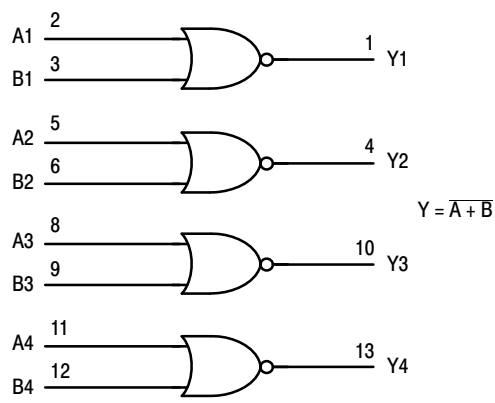
Figure 1. LOGIC DIAGRAM
