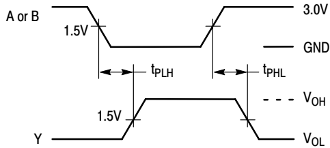
Figure 3. Switching Waveforms
