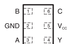
YFP OR YZP PACKAGE (TOP VIEW)
