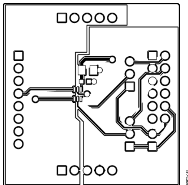
Figure 15. Component Placement Drawing
