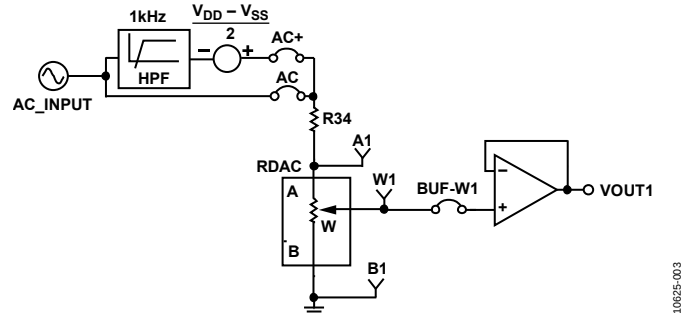
Figure 3. AC Signal Attenuator
