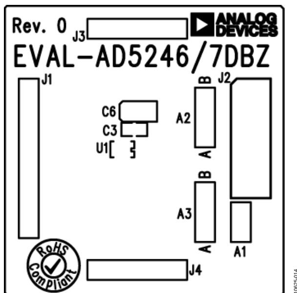
Figure 14. Component Side View
