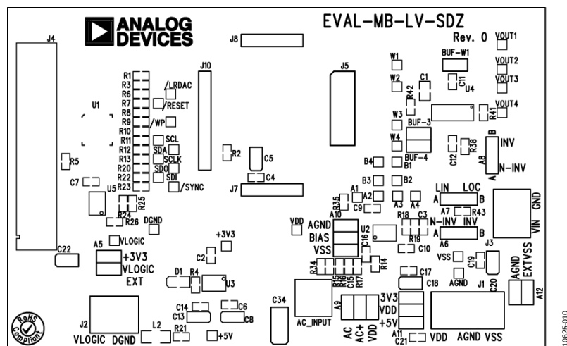
Figure 10. Component Side View
