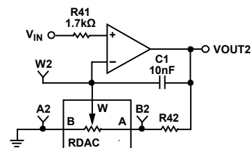
Figure 4. Pseudologarithmic Noninverting Amplifier
