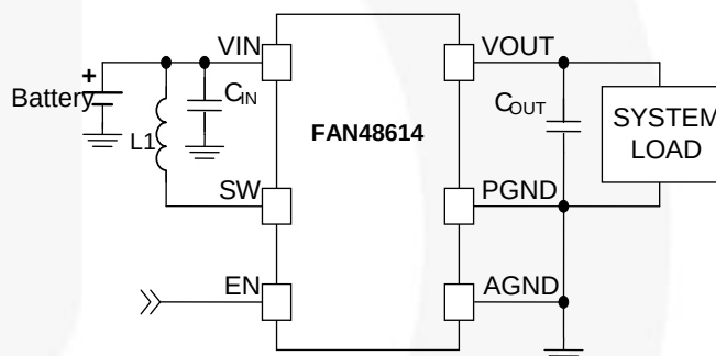
Figure 1. Typical Application
