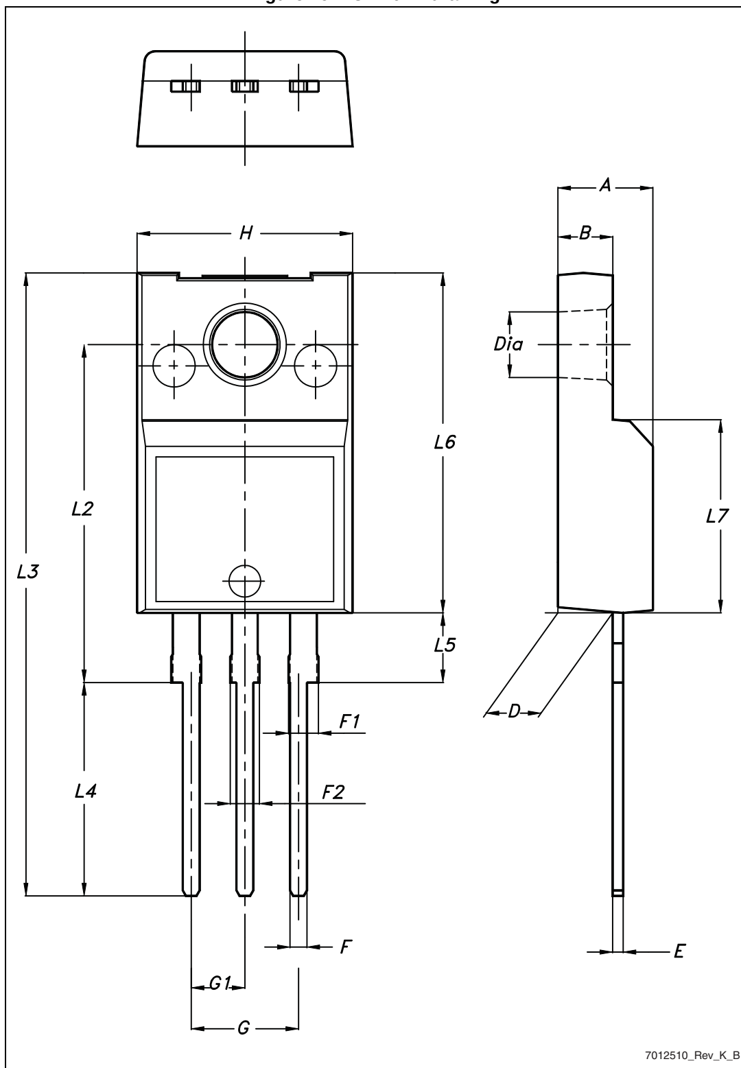
Figure 29. TO-220FP drawing
