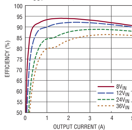
5V OUT Efficiency
