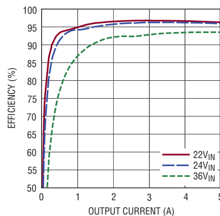
18V OUT Efficiency
