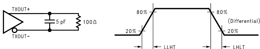
Figure 5. DS90C387R LVDS Output Load and Transition Times
