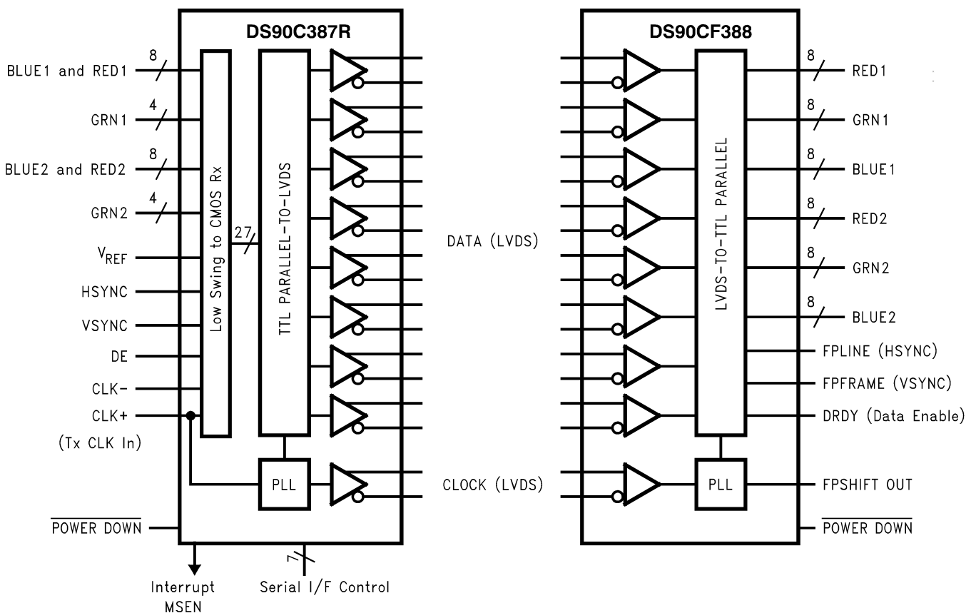
Figure 1. DS90C387R
