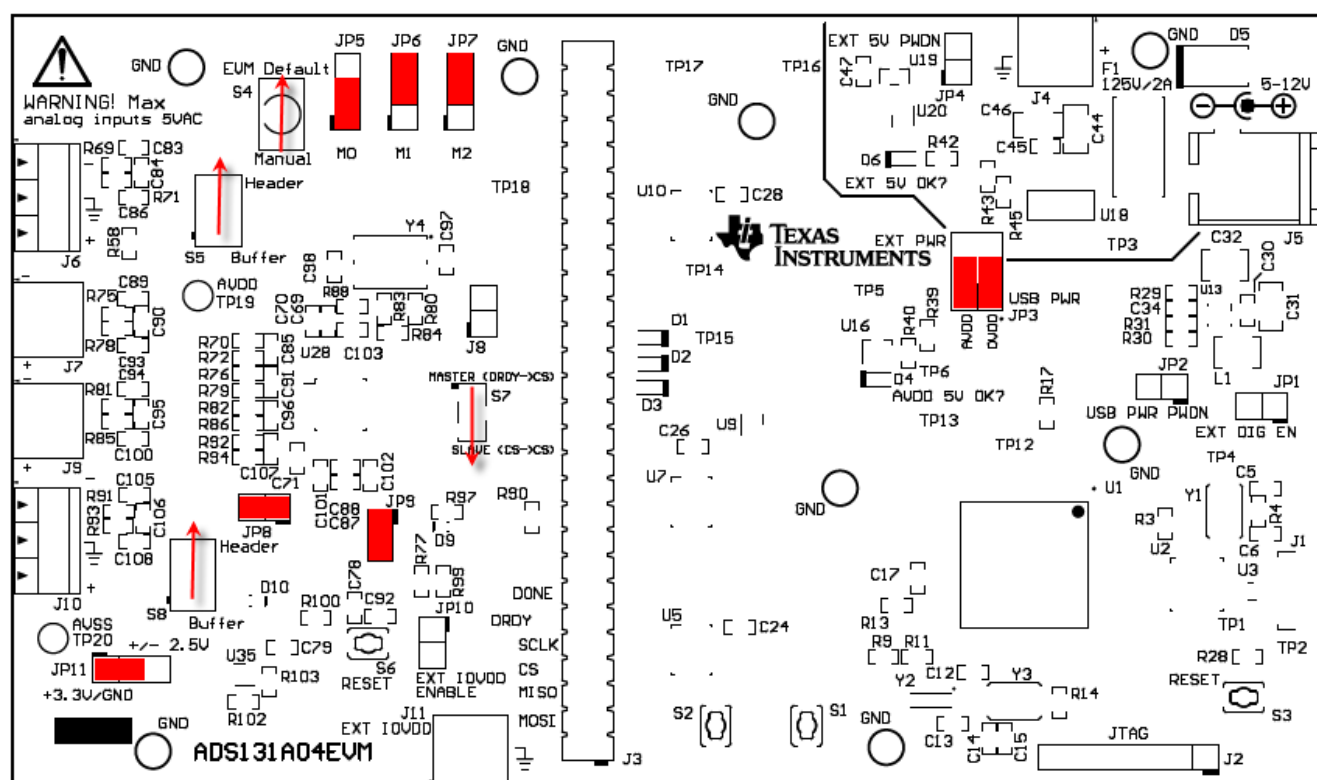
Figure 2. ADS131A04 EVM
