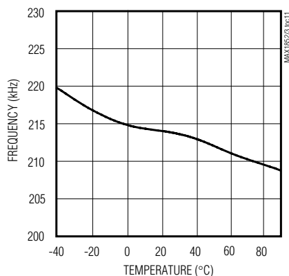
MAX1853 CHARGE-PUMP FREQUENCY vs. TEMPERATURE
