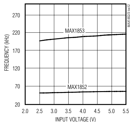
CHARGE-PUMP FREQUENCY vs. INPUT VOLTAGE
