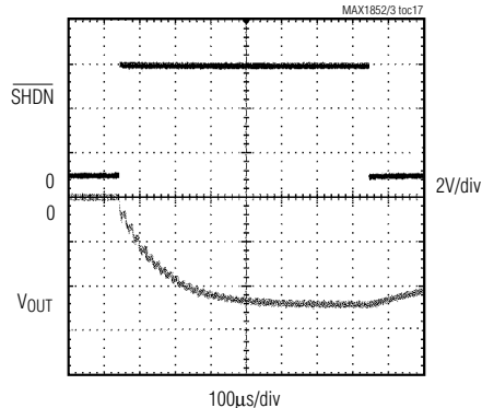
MAX1852 STARTUP FROM SHUTDOWN
