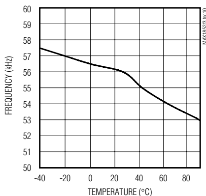
MAX1852 CHARGE-PUMP FREQUENCY vs. TEMPERATURE
