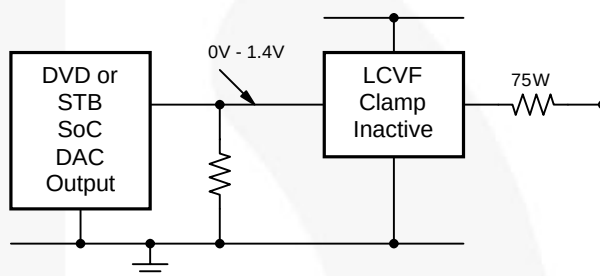
Figure 14. DC-Coupled Inputs and Outputs
