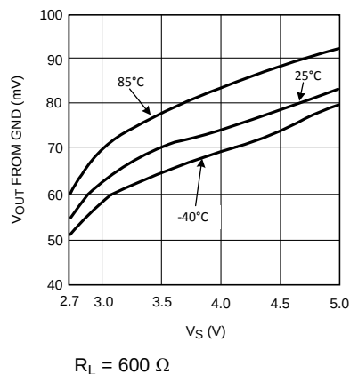
Figure 6. Output Negative Swing vs Supply Voltage
