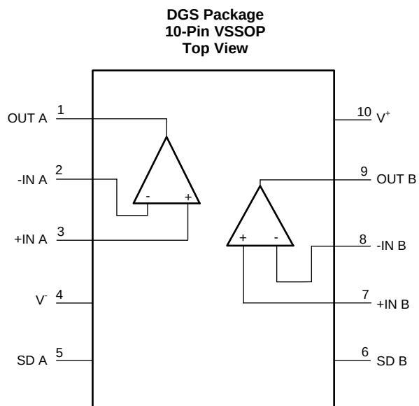
Pin Functions: VSSOP Package
