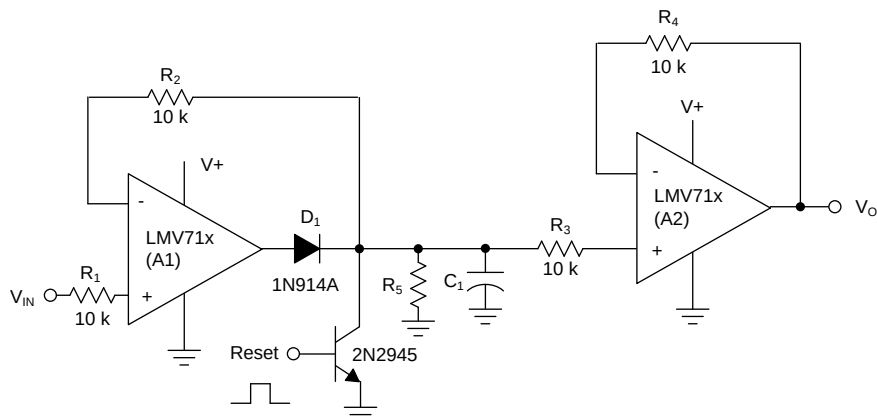
Figure 36. Peak Detector Schematic
