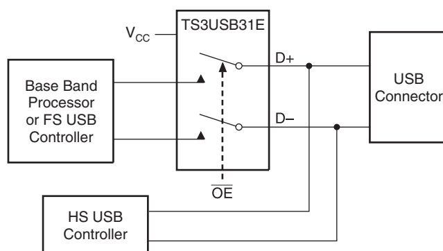
Figure 13. Application Diagram
