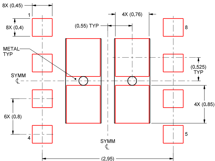
SOLDER PASTE EXAMPLE BASED ON 0.125 mm THICK STENCIL EXPOSED PAD 85% PRINTED SOLDER COVERAGE BY AREA SCALE:25X
