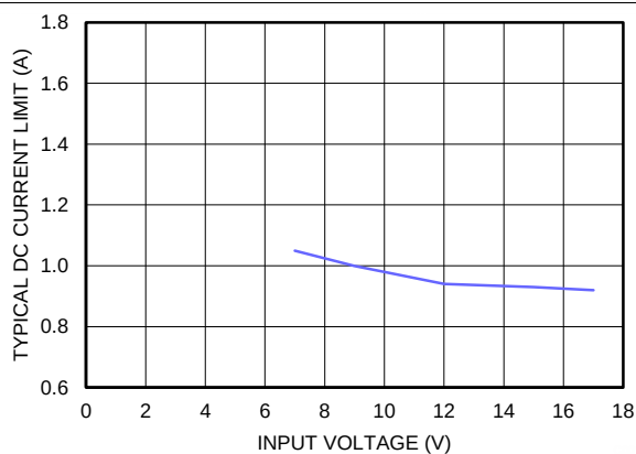
Figure 77. Typical Current Limit V_{OUT} = 5.0 V, T_A = 85^\circ\text{C}
