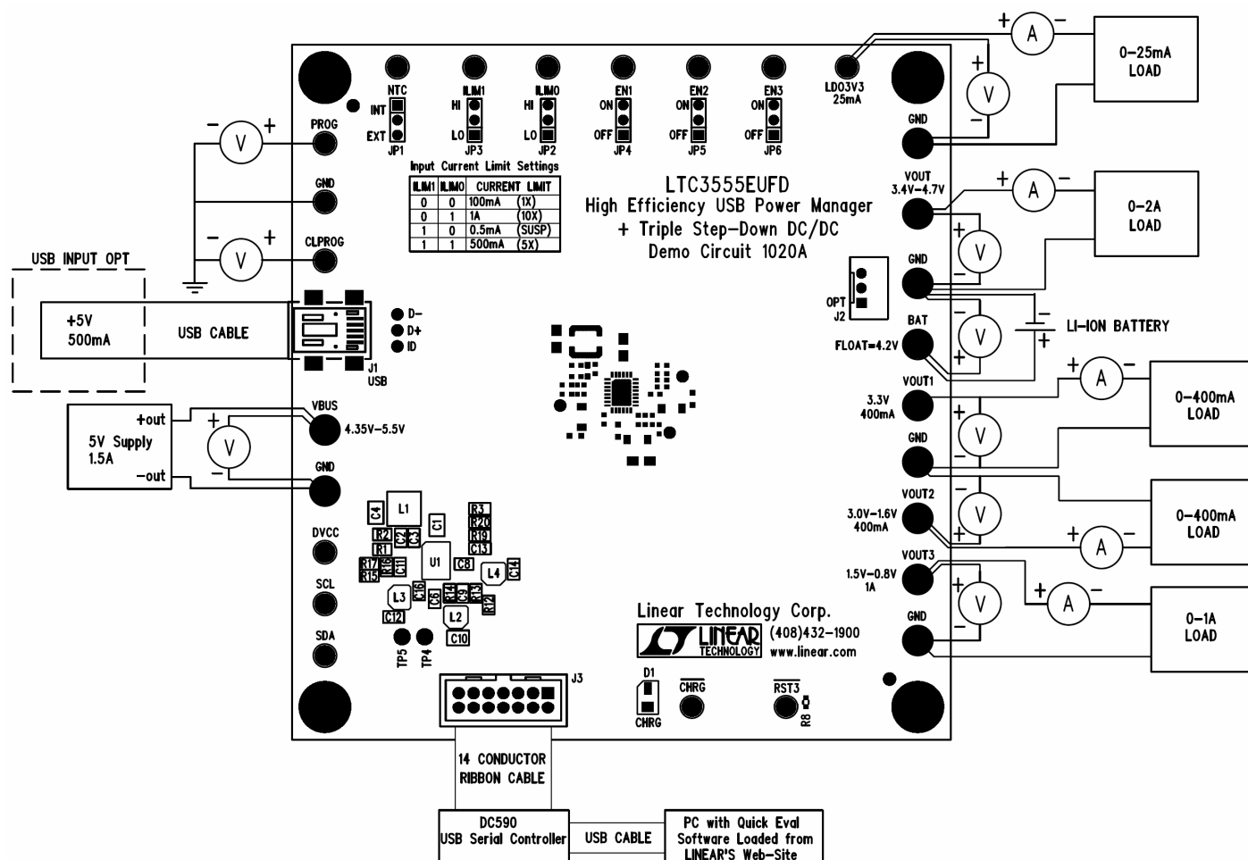
FIGURE 2: Proper Measurement Equipment Setup for DC1020
