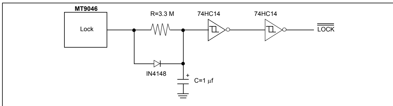
Figure 11 - Time-constant Circuit
