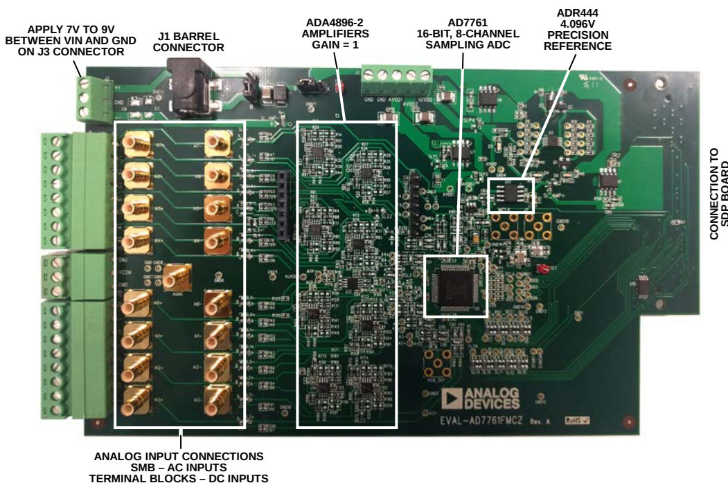
Figure 1. Evaluation Board
