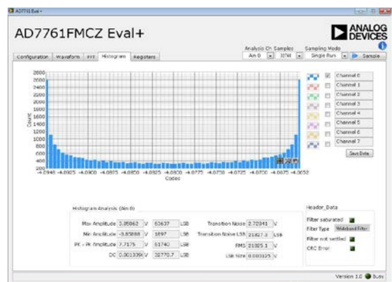
Figure 21. Histogram Tab
