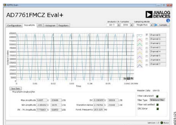
Figure 19. Waveform Tab
