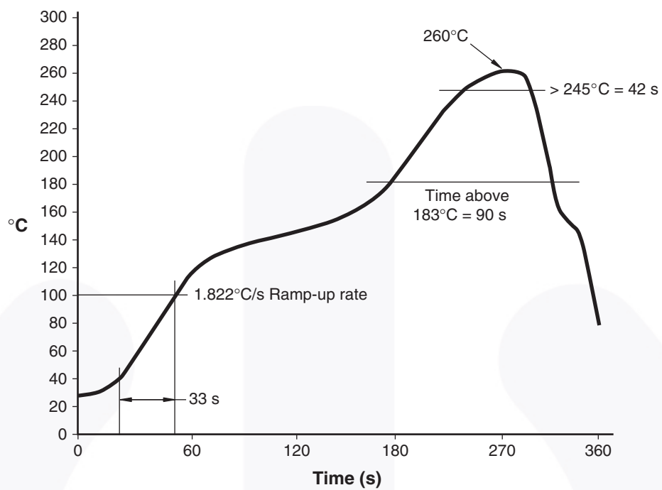
Figure 9. Reflow Profile
